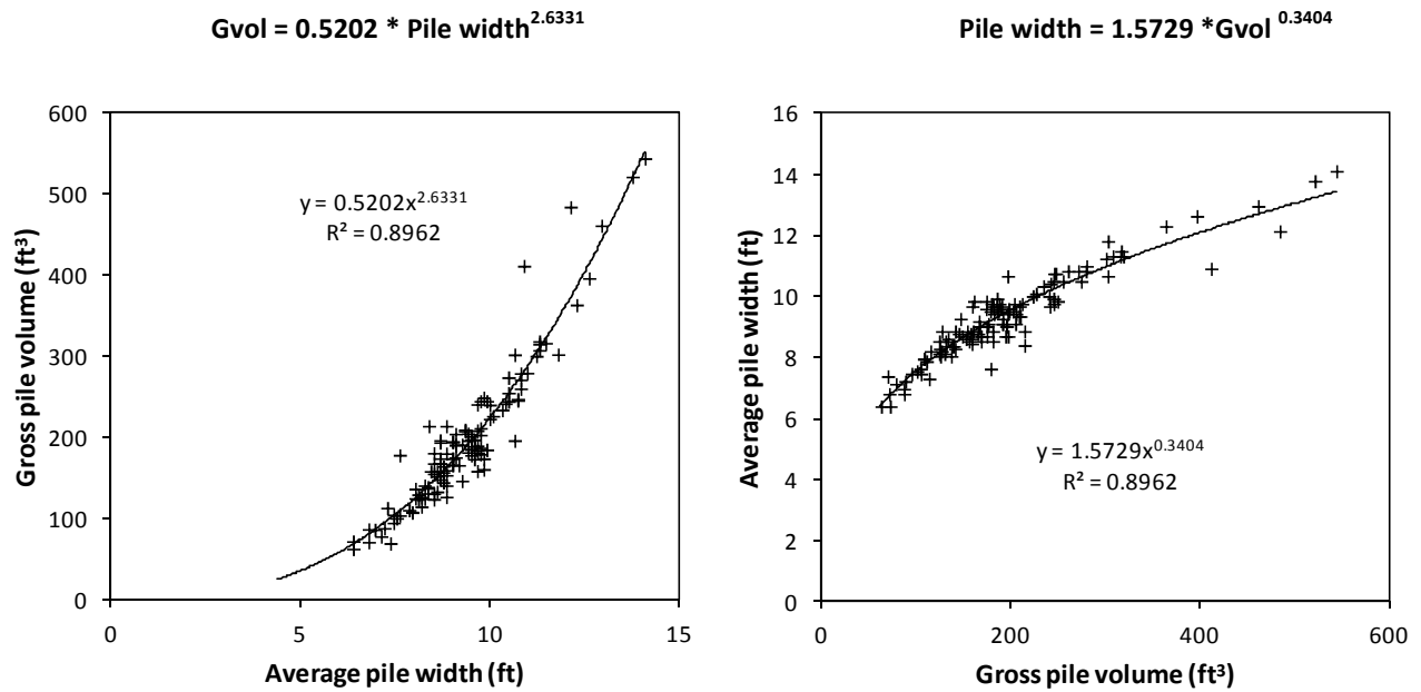
Figure 3. Relationship between burn pile width (average of width and length measurements) and gross pile volume calculated by entering width, length, and height measurements into the pile calculator (Wright et al. 2009).
