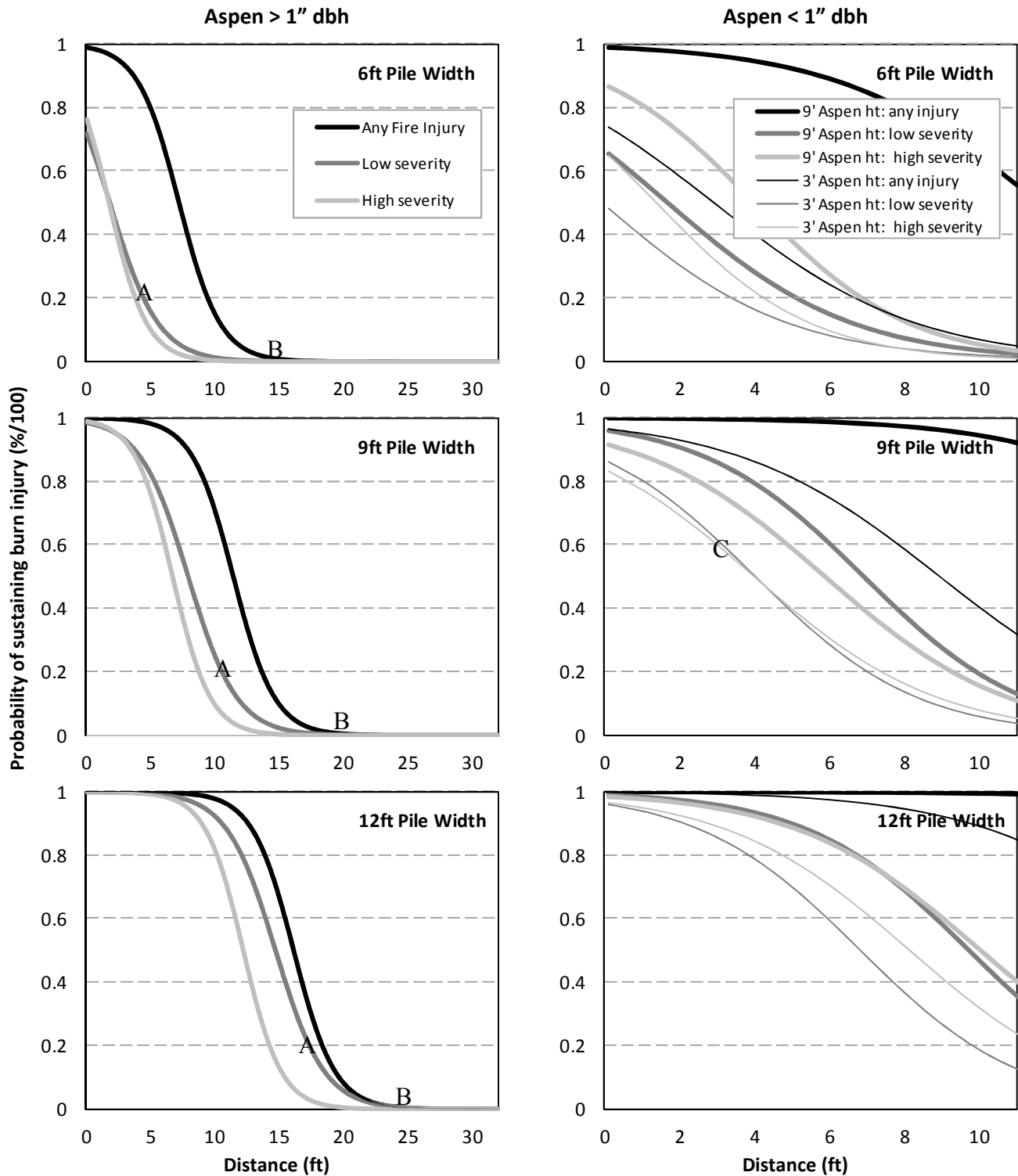
Figure 4. Predicted probability of aspen injury related to pile width and distance from burn pile (e.g. where probability of 0.5 = 50% chance of injury) based on pile and injury data from fall burning in 2011 at one site (WA38). Scenario A: 20% probability of “low severity” injury; B: 0% probability of “Any injury”; C: 60% probability of “high severity” injury to small trees.
