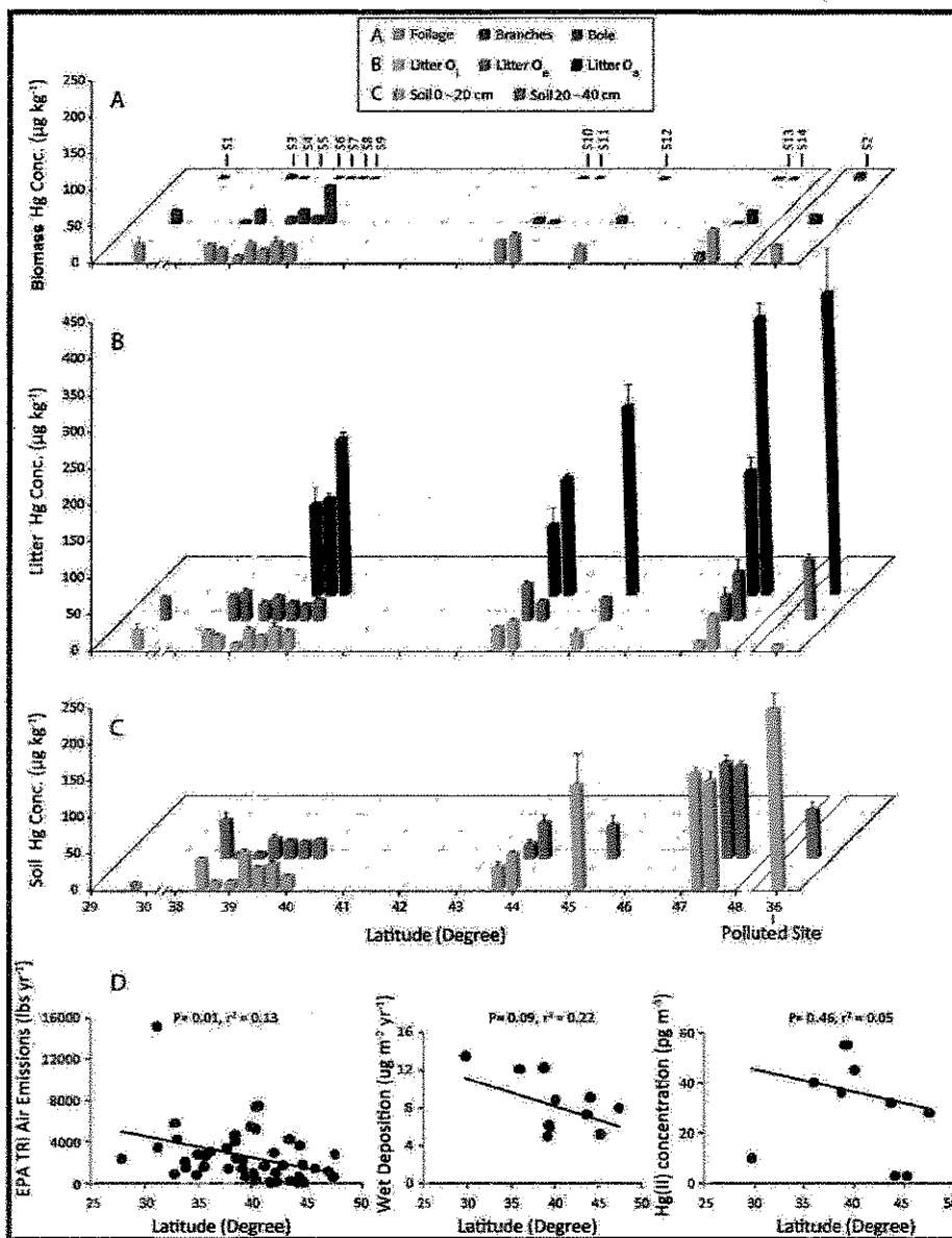
Figure 1. Hg concentrations (in \mu\text{g kg}^{-1} ) of major ecosystem components (Panels A–C). Each bar represents average concentration plus standard error of four replicate plots. Sites are numbered S1–S14 according to site names in SI Figure S1 and Table S1 and are ordered by latitude (exception of site S2 which is influenced by local Hg pollution). A: Hg concentrations in aboveground biomass tissues. Values represent average of dominant tree species on sites (i.e., 1–4 species per site). B: Litter Hg concentrations, separated into Oi (fresh), Oe (partially decomposed), and Oa (strongly decomposed) layer. C: Concentrations in soils, averaged for top 0–20 cm and 20–40 cm depths. D: Latitudinal trends of atmospheric pollution proxies. These data were extrapolated from other data sets. 11,13,21 For wet deposition and Hg(II) concentrations, only values for the 13 sites were extrapolated.
