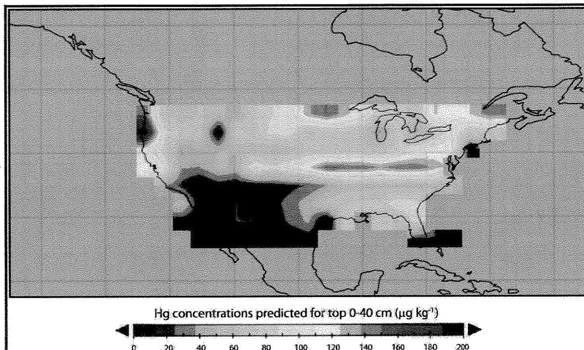
Figure 3. Spatial extrapolation of top soil (0–40 cm) Hg concentrations based on multiregression modeling using independent variables latitude, precipitation, soil C content, and clay content ( r^2 = 0.88 ; SI Table 2A). Underlying soil C distribution was calculated using the Community Land Model (CLM) with the Carnegie-Ames-Stanford Approach to simulate equilibrium carbon densities in soils. Note that due to grid resolution, the map extrapolates Hg concentrations also over areas with no soils such as the Great Lakes and along coastal waters.
