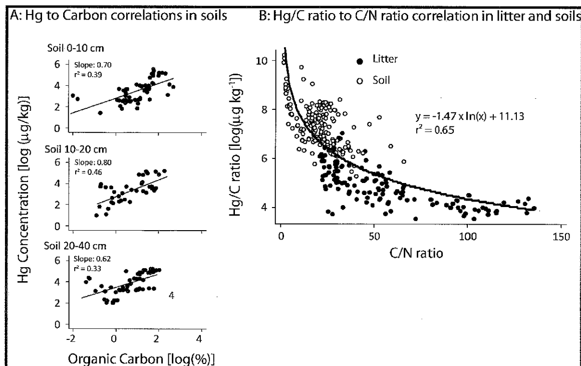
Figure 2. Hg to C relationships observed in soils and litter. A. Linear correlations between soil Hg and C concentrations for all samples taken from the 13 remote sites at depths of 0–10 cm, 10–20 cm, and 20–40 cm. We used multiregression analyses (with dummy variables) to test for differences in slopes and intercepts of regressions between Hg and C for various soil depths. B. Relationships between Hg/C ratios in all litter and soil samples (0–40 cm) and respective C/N ratios of samples.
