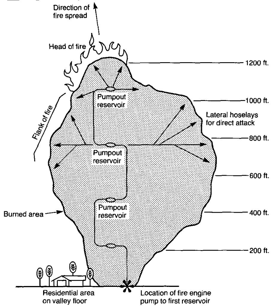
Figure 3—Diagram of use of equipment to fight a typical frontal fire.
