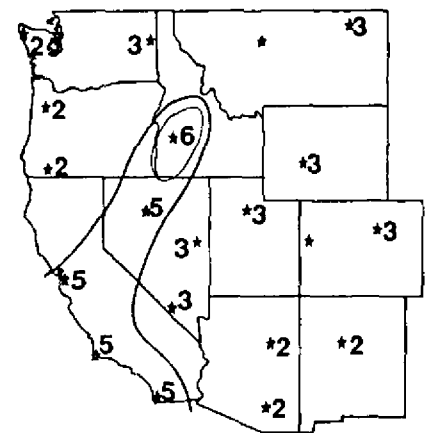
Figure 6 —Haines Index map for 0600 MDT, July 29, 1989. Solid contour indicates a value of 5 or greater; dashed contour, 6. (The Great Falls, MT, and Grand Junction, CO, data are missing for July 19, 1989.)
