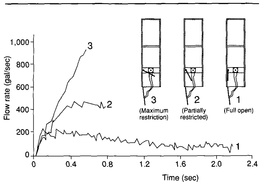
Figure 5—Diagram of one approach to achieving variable flow rate in a conventional tank.
