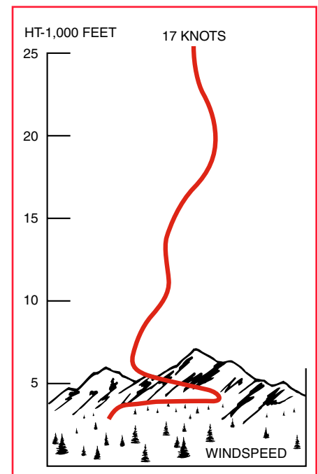
Figure 4—Wind profile showing a low-level jet. Low-level jets usually occur over relatively flat terrain just above the nighttime inversion layer, but they can also occur under other conditions. Haines and Kuehnast (1970) attributed the blowup fires of 1871 to wind shear and turbulence caused by low-level jets associated with an approaching cold front.
