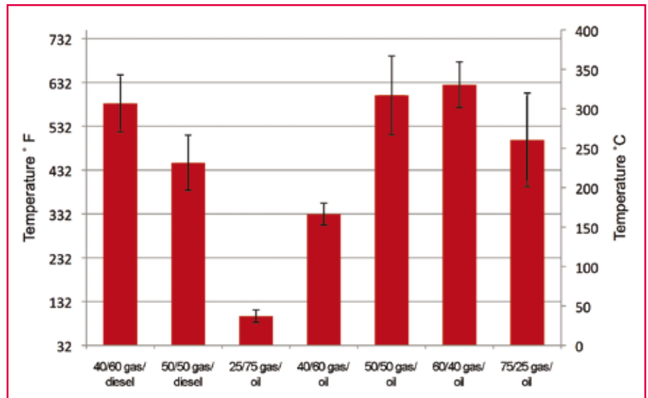
Figure 2—Average maximum burn temperature of fuel mixtures tested in the laboratory. Baseline results for the gasoline-diesel fuel mixtures are on the left, and results for the various gasoline-waste oil mixtures are on the right. Error bars indicate standard error.
