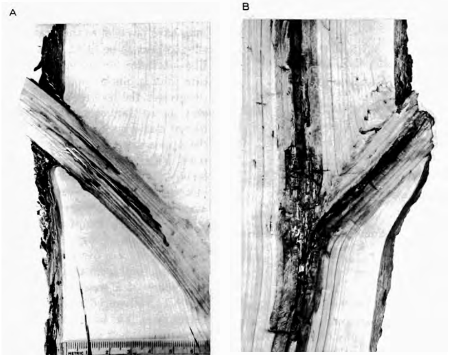
FIGURE 3.—Radial-longitudinal sections of the trunks of immature trees showing: A, Red rot that extended into the knot—the central position of the longest column indicates that the red rot fungus made more rapid progress through the pith cavity than in the wood; B, red rot that reached the trunk heartwood through the pith cavity of the knot.
