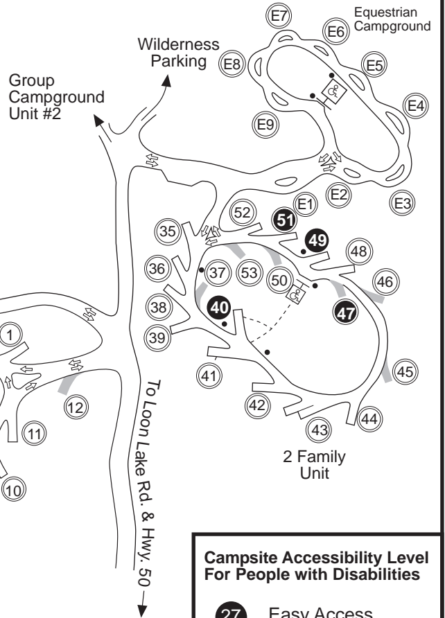
Location Map
