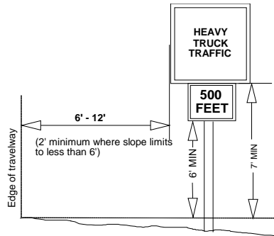
Figure 1: Sign Placement
