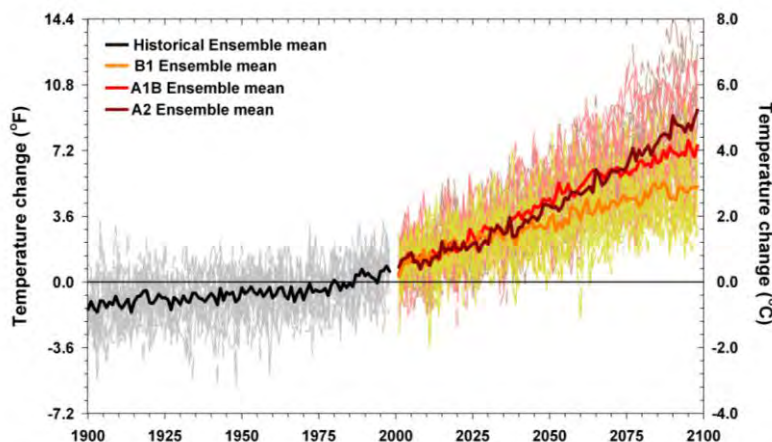
Figure 1. Northern Rockies and 2001-2099 (color). Heavy lines are ensemble (multiple climate model) averages for B1, A1B, and A2 emissions scenarios.
