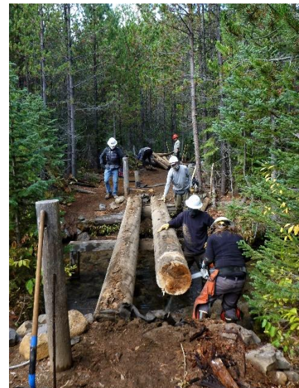
Volunteers with the Central Oregon Nordic Club and Central Oregon Trails Alliance, along with FS staff, remove an old bridge on the Tumalo Creek Bridge. A new bridge is currently being constructed.
