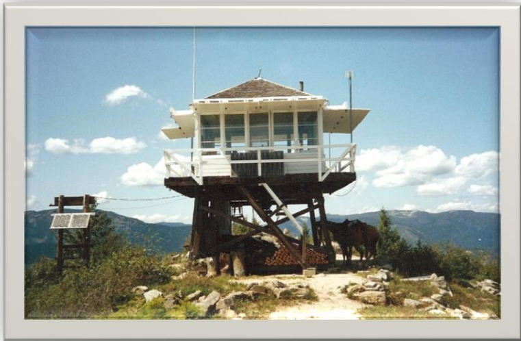
Shissler Lookout, 1992. This treated timber L-4 tower is 10' tall with a hip roof. Built in 1953, Shissler Lookout remains staffed and is located three miles north of Moose Creek Ranger Station on the Moose Creek Ranger District within the Selway-Bitterroot Wilderness. Cindy Schacher photo
