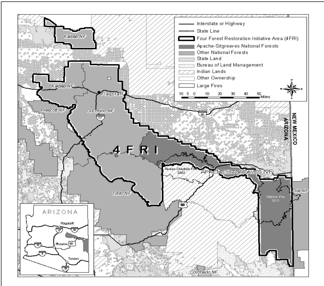
Map 2. Four Forests Restoration Initiative project scale in Northern Arizona
