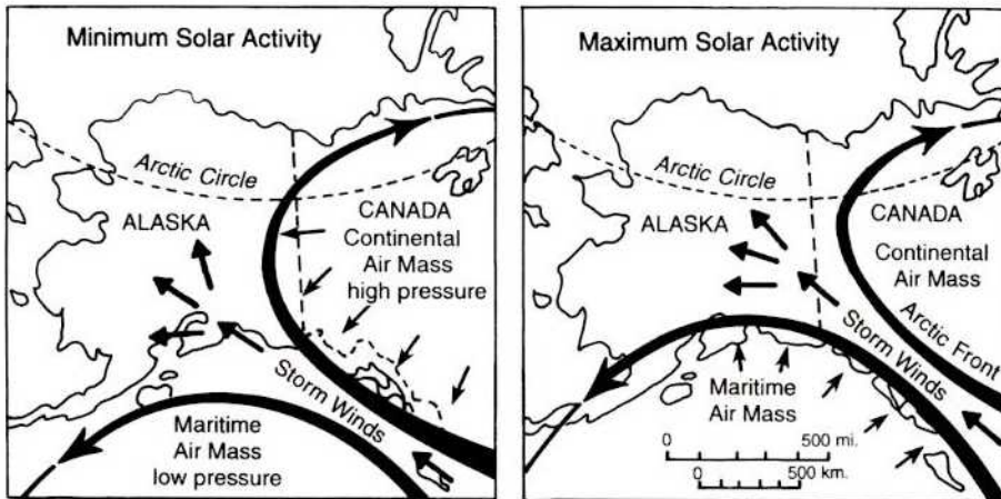
Fig. 5. Typical influences of maritime air mass (right) in southeast Alaska and its displacement offshore by the continental air mass (left) (MILLER 1985). These models may be used to understand general climatic patterns that are influenced by cycles of solar radiation or sudden shifts to frigid temperatures during winter in southeast Alaska
