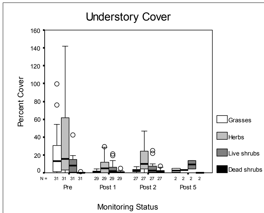
Figure 19 – Understory cover associated with prescribed fire treatment in Ponderosa and Yellow Pine.
