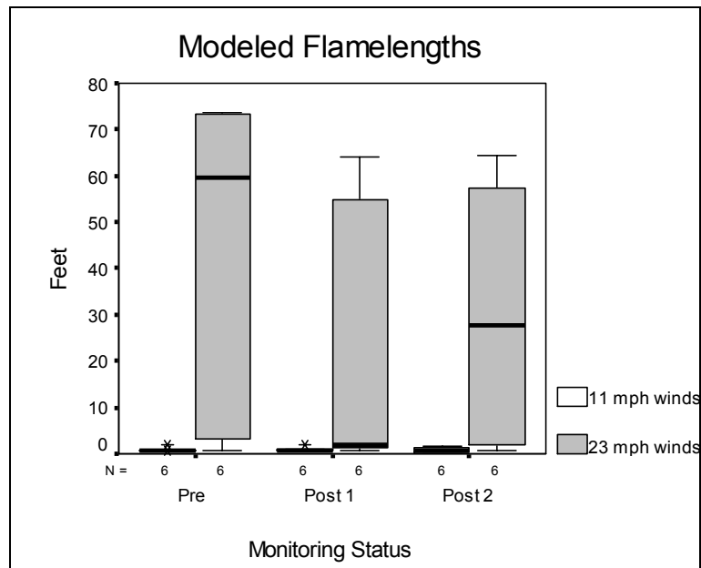
Figure 41 – Modeled flamlengths measurements associated with mechanical treatment in Red Fir.
