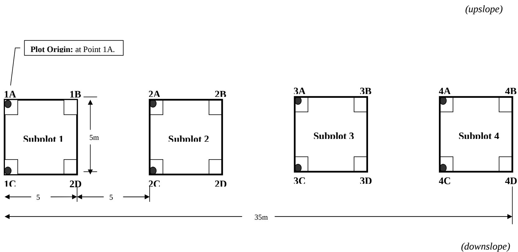
Figure A-2 – Chaparral Plot Layout
