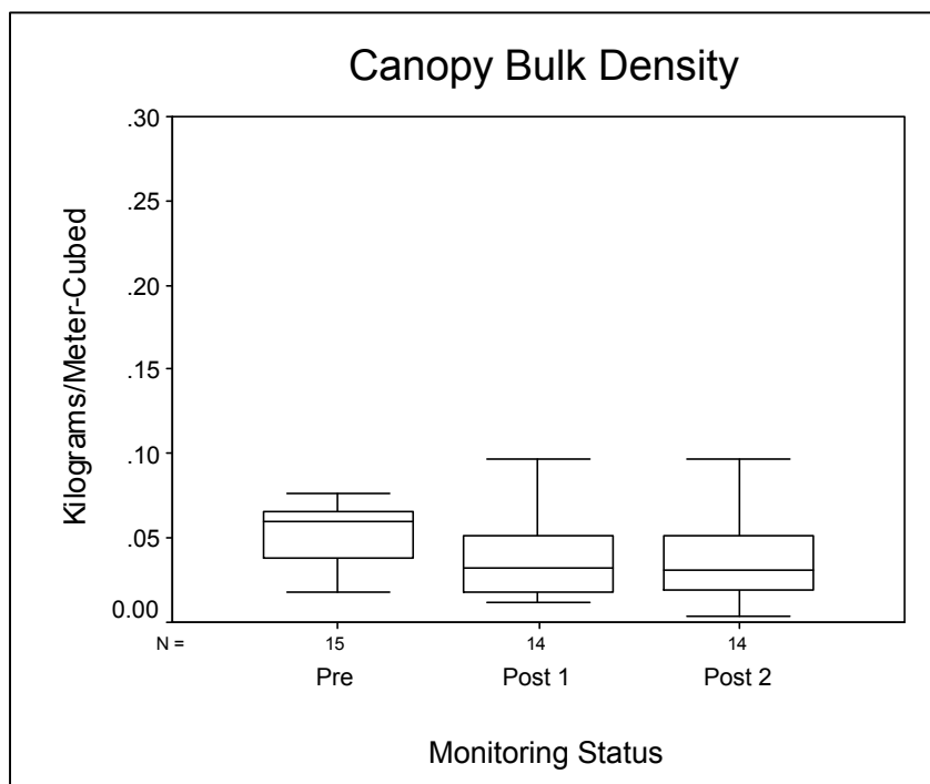
Figure 33 – Canopy bulk density measurements associated with mechanical treatment in Ponderosa and Yellow Pine.
