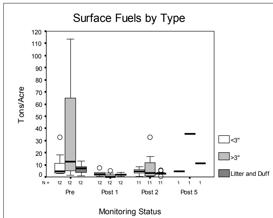
Figure 6 – Surface fuels by type associated with prescribed fire treatments in short needle dominated, Douglas Fir and White Fir type.
