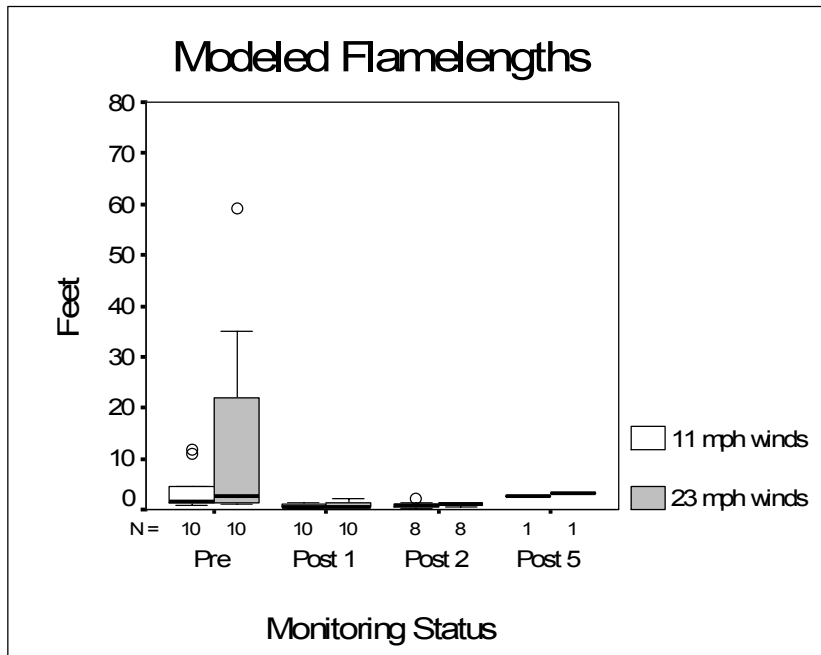
Figure 9 – Modeled flame length measurements associated with prescribed fire in Douglas Fir and White Fir types.
