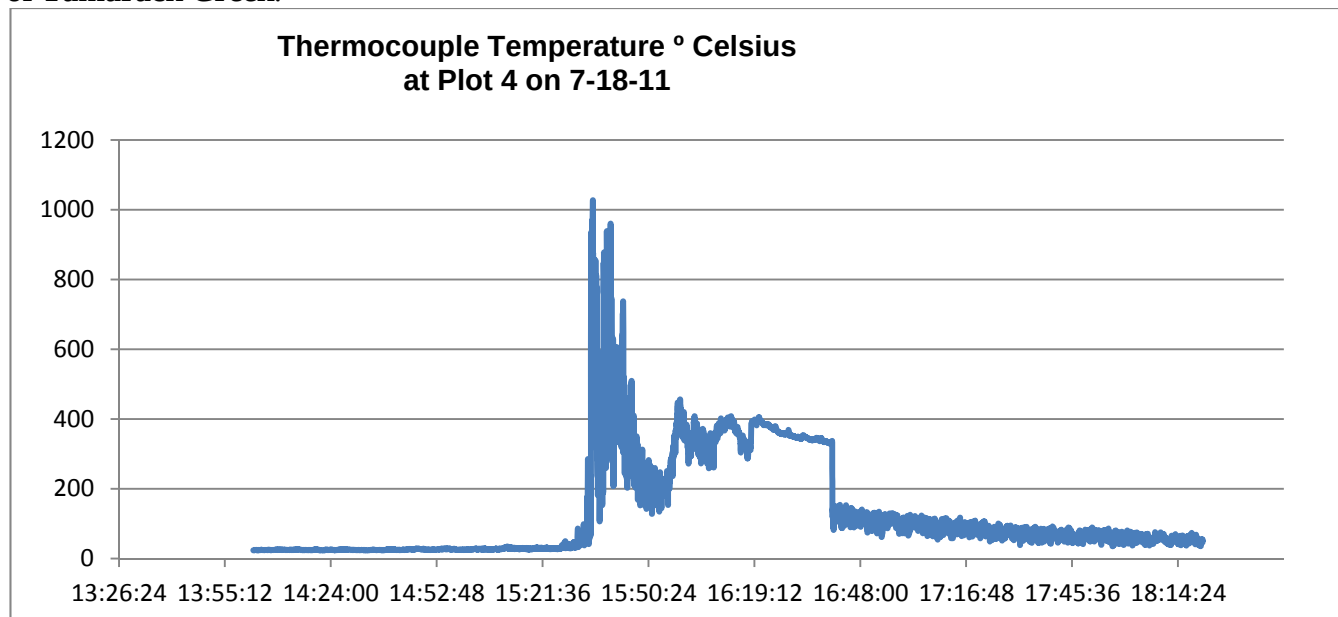
Figure 14: Thermocouple temperature graph of portion of temperatures measured at plot 4, south of Tamarack Creek.
