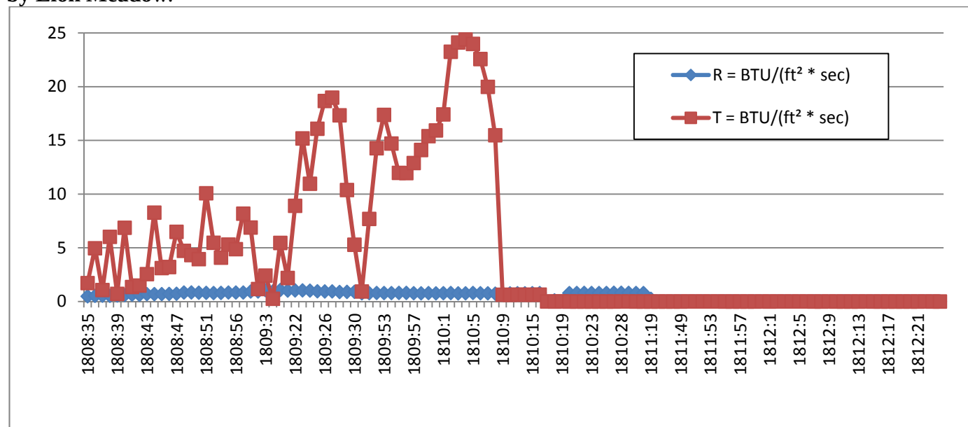
Figure 13: Heat flux graph of portion of temperatures measured at plot 6, near the private cabins by Lion Meadow.
