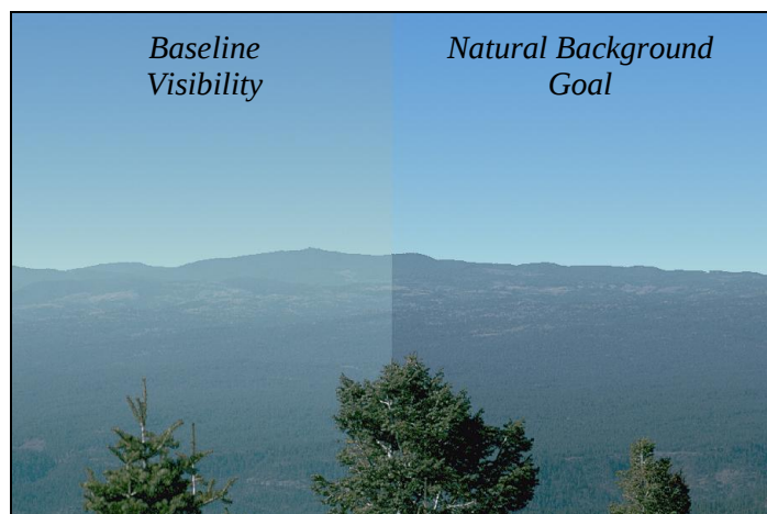
Figure 1: Baseline vs. Natural Background Visibility at Mount Baldy Wilderness Area in Arizona
