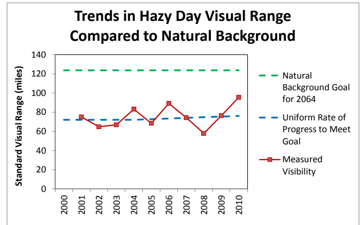
Figure 4: Changes in Visibility as Compared to Uniform Rate of Progress and Natural Background Goal at Mount Baldy
