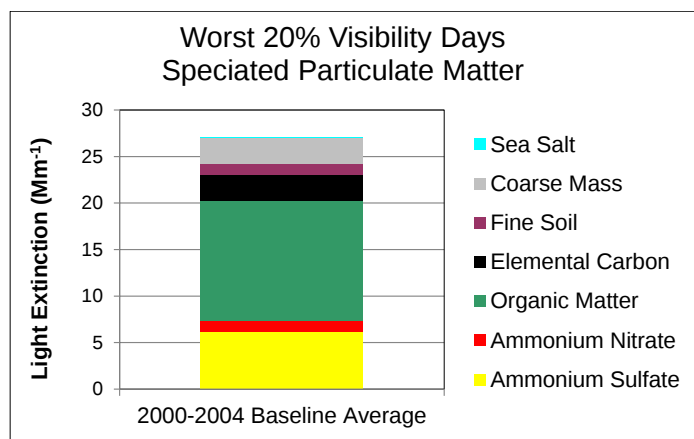
Figure 3: Composition of Particulate Matter on Hazeiest Days at Mount Baldy Wilderness Area
