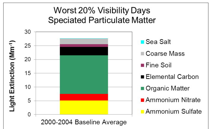
Figure 3: Composition of Particulate Matter on Haziest Days at the Desolation and Mokelumne Wilderness Areas
