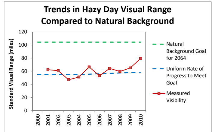
Figure 4: Changes in Visibility as Compared to Uniform Rate of Progress and Natural Background Goal at Mount Hood
