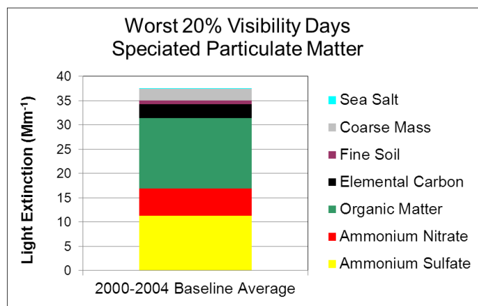
Figure 3: Composition of Particulate Matter on Haziest Days at Mount Hood Wilderness Area
