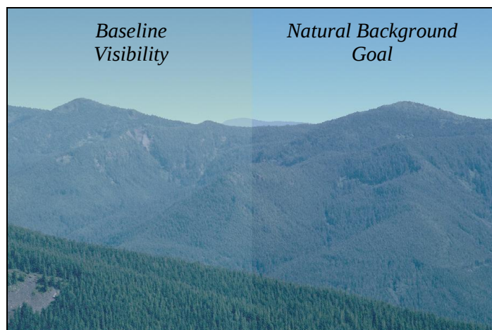
Figure 1: Baseline vs. Natural Background Visibility at Mount Hood Wilderness Area in Oregon
