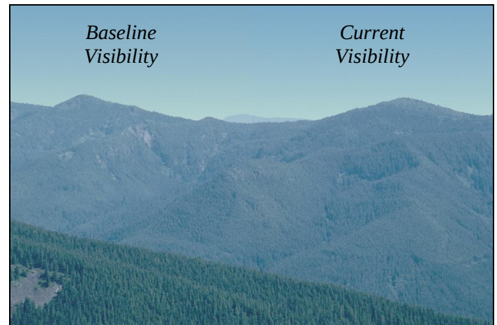
Figure 5: Computer Generated Approximation of the Visibility Improvement at Mount Hood Wilderness Area
