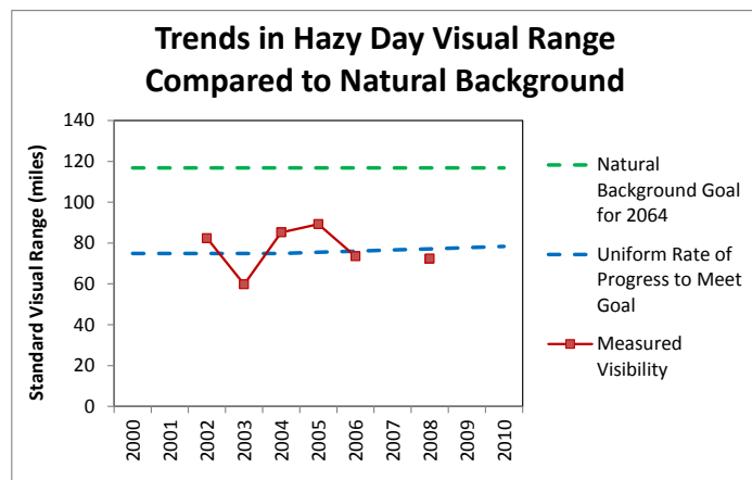
Figure 4: Changes in Visibility as Compared to Uniform Rate of Progress and Natural Background Goal at North Absaroka and Washakie
