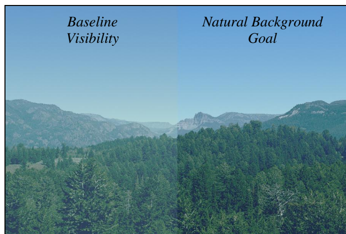
Figure 1: Baseline vs. Natural Background Visibility at Teton Wilderness Area in Wyoming
