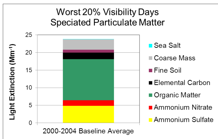
Figure 3: Composition of Particulate Matter on Hazeiest Days at the North Absaroka and Washakie Wilderness Areas
