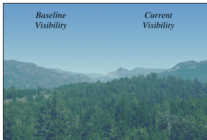
Figure 5: Computer Generated Approximation of the Visibility Improvement at Teton Wilderness Area
