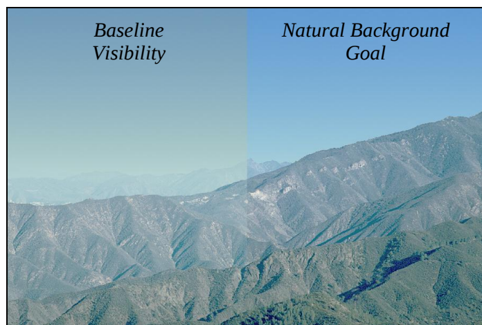
Figure 1: Baseline vs. Natural Background Visibility at San Rafael Wilderness Area in California
