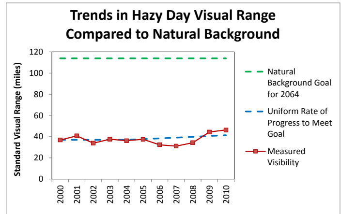
Figure 4: Changes in Visibility as Compared to Uniform Rate of Progress and Natural Background Goal at San Rafael
