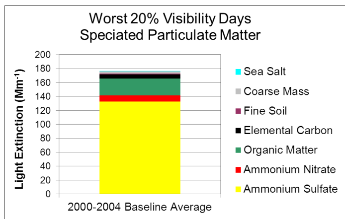
Figure 3: Composition of Particulate Matter on Hazeiest Days at Sipsey Wilderness Area
