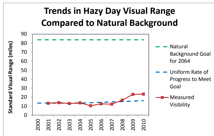
Figure 4: Changes in Visibility as Compared to Uniform Rate of Progress and Natural Background Goal at Sipsey
