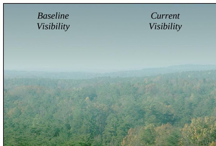
Figure 5: Computer Generated Approximation of the Visibility Improvement at Sipsey Wilderness Area
