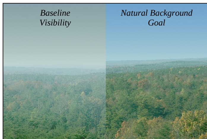
Figure 1: Baseline vs. Natural Background Visibility at Sipsey Wilderness Area in Alabama
