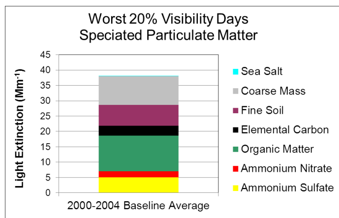
Figure 3: Composition of Particulate Matter on Hazeiest Days at Sycamore Canyon Wilderness Area
