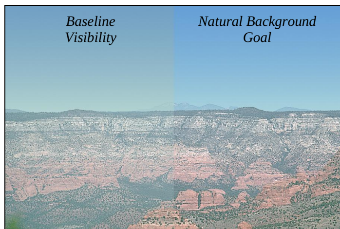
Figure 1: Baseline vs. Natural Background Visibility at Sycamore Canyon Wilderness Area in Arizona
