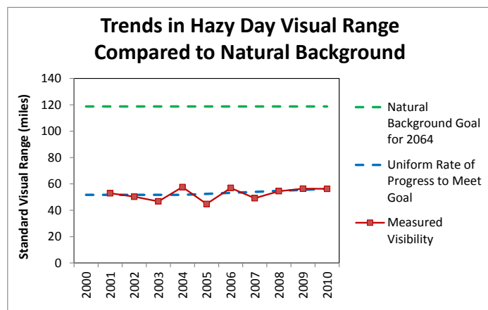
Figure 4: Changes in Visibility as Compared to Uniform Rate of Progress and Natural Background Goal at Sycamore Canyon
