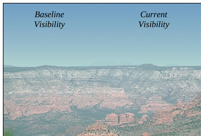
Figure 5: Computer Generated Approximation of the Visibility Improvement at Sycamore Canyon Wilderness Area
