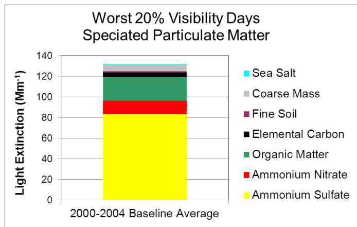
Figure 3: Composition of Particulate Matter on Haziest Days at Upper Buffalo Wilderness Area
