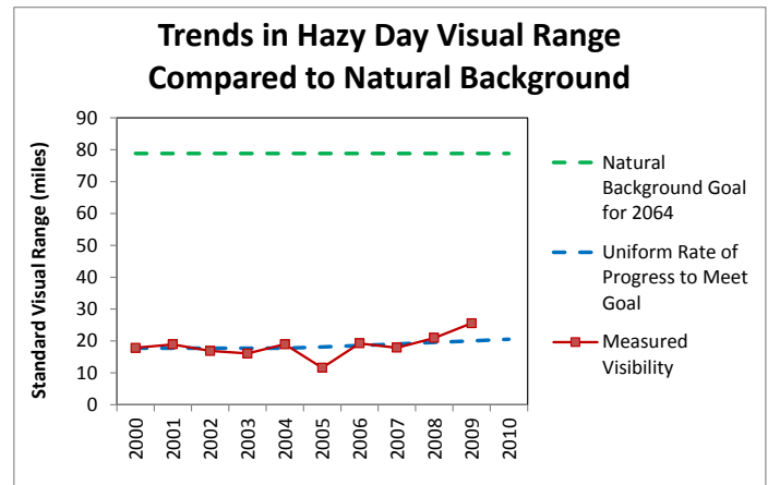
Figure 4: Changes in Visibility as Compared to Uniform Rate of Progress and Natural Background Goal at Upper Buffalo
