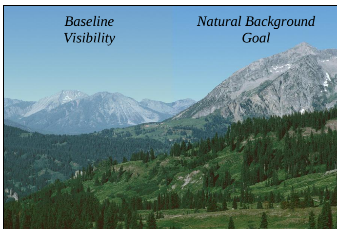
Figure 1: Baseline vs. Natural Background Visibility at West Elk Wilderness Area in Colorado
