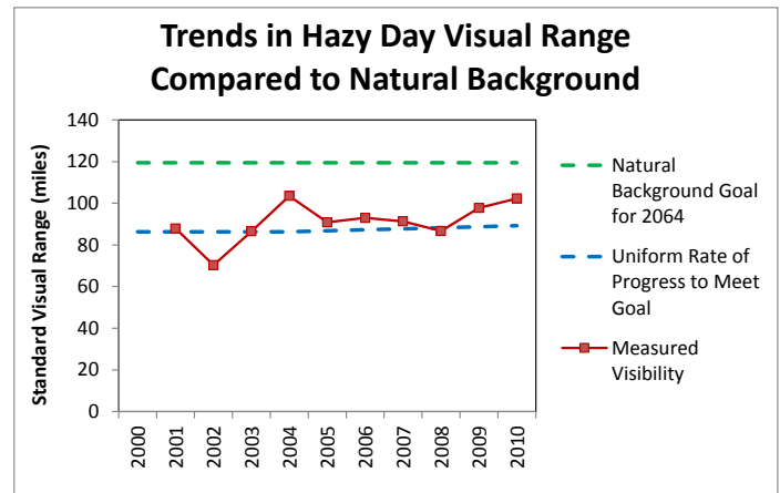
Figure 4: Changes in Visibility as Compared to Uniform Rate of Progress and Natural Background Goal at Eagles Nest, Flat Tops, Maroon Bells-Snowmass, and West Elk
