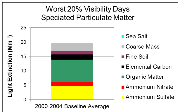
Figure 3: Composition of Particulate Matter on Hazeiest Days at the Eagles Nest, Flat Tops, Maroon Bells-Snowmass, and West Elk Wilderness Areas
