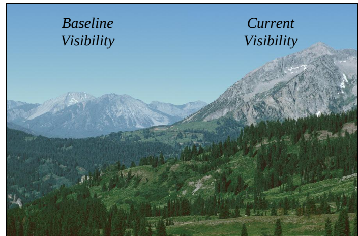
Figure 5: Computer Generated Approximation of the Visibility Improvement at West Elk Wilderness Area
