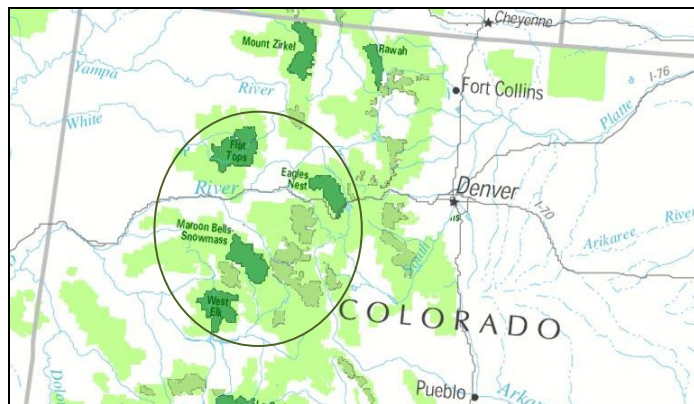
Figure 2: Location of Eagles Nest, Flat Tops, Maroon Bells-Snowmass, and West Elk Wilderness Areas
