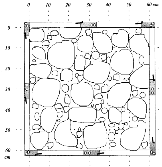
Figure 1. Eight-piece 60 by 60 cm collapsible sampling frame constructed from aluminum bars. An adjustable grid of thin white elastic bands are stretched horizontally and vertically across the frame to define the exact particles to sample. When the frame is placed onto the stream bed, the elastic bands stretch across the cobbles that protrude above the bed.
