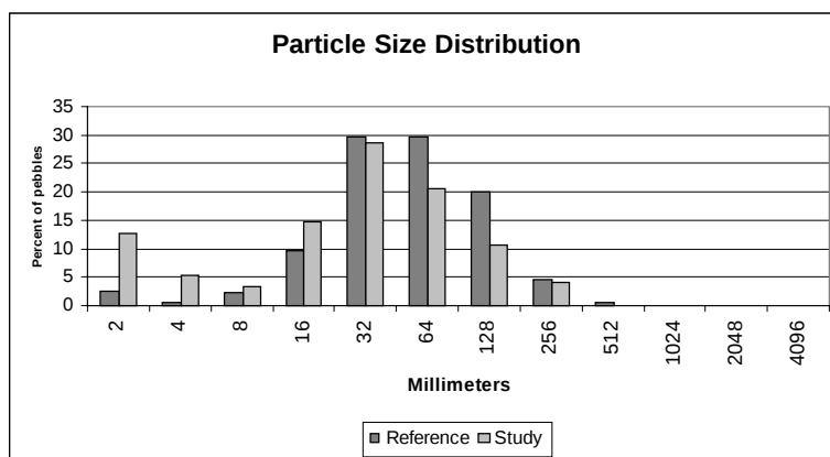
Figure 2. An example of particle size tabulations and particle size distribution and histogram plots automatically generated by the analysis spreadsheets.
