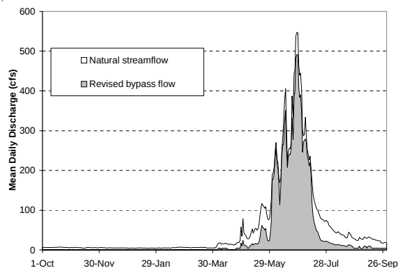
Figure 3. The revised bypass flow regime is shown in light gray. This flow regime requires passing most of the channel-forming flows through the bypass reach and mimics the natural hydrograph. A small proportion of the flow is always allocated to power production making it possible to generate power continuously while bypassing most of the water to meet geomorphic objectives.
