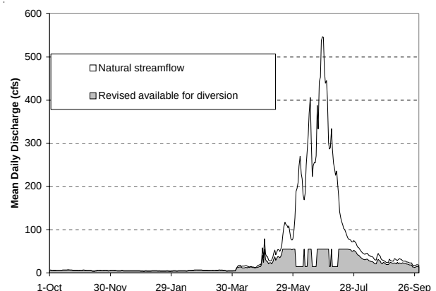
Figure 5. The revised streamflow available for diversion and power production is shown in light gray. This flow regime provides about the same amount of water for power production as the former structure; however, water is proportioned between by-pass and power production throughout the year allowing continuous generation of electricity.
