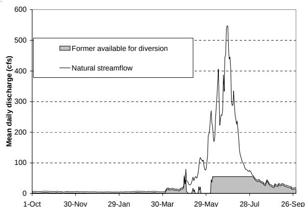
Figure 4. The former streamflow available for diversion and power production is shown in light gray. The facility has a maximum capacity of 55 cfs, however, water is unavailable for power production during a portion of the rising limb of the hydrograph because of the structure of the bypass flow regime.
