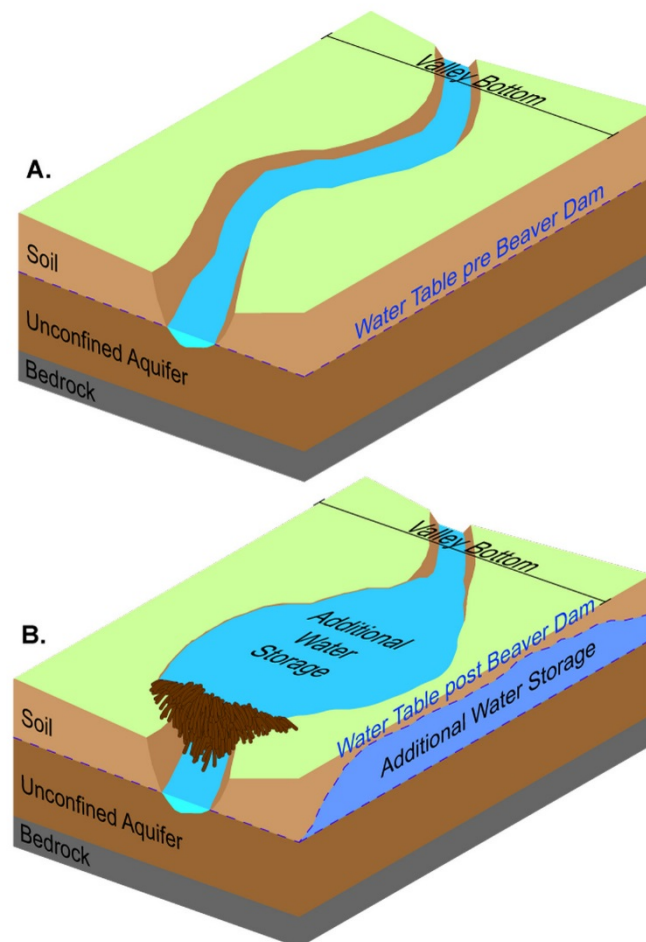
Figure 3: Conceptual illustration of water storage additions pre-beaver dam (A) and post-beaver dam (B) construction to above and below ground water storage.
