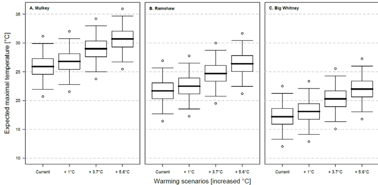
Figure 6: Current water temperatures and predicted future temperatures under 3 different climate warming scenarios ( PlosOne article ) in Mulkey, Ramshaw, and Big Whitney meadows, Golden Trout Wilderness, California.
