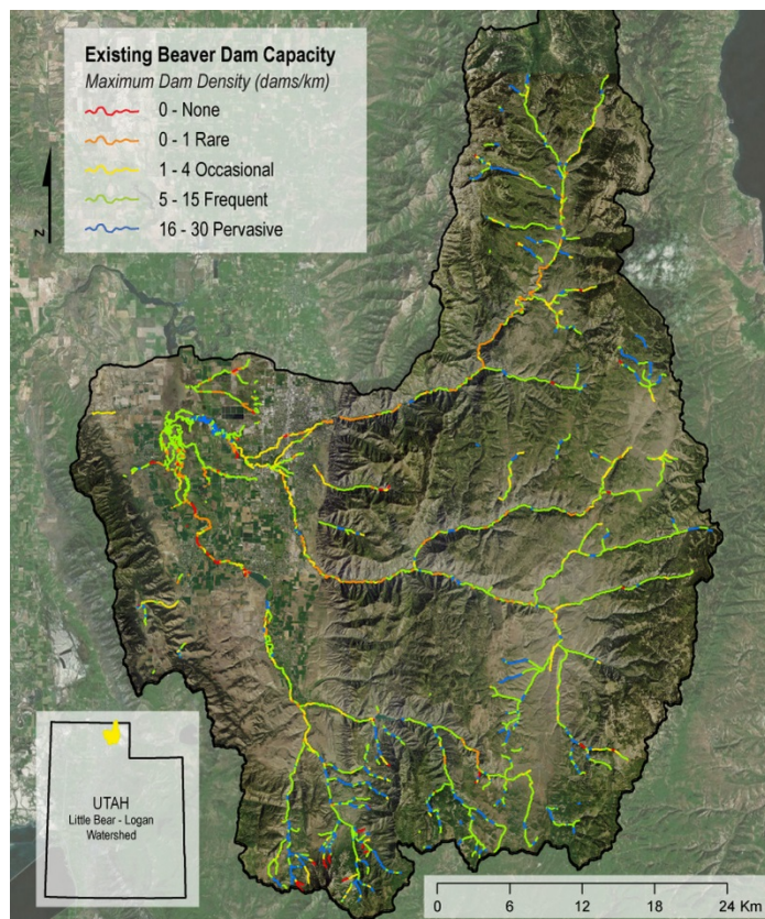
Figure 2: Modeled beaver dam capacity estimates from the Beaver Restoration Assessment Tool (BRAT) for the Little Bear-Logan River watershed in northern Utah.
