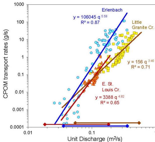
Figure 10: CPOM transport versus unit discharge, E. St. Louis, Little Granite, and Erlenbach Creeks.
