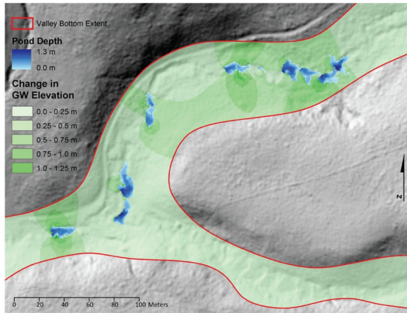
Figure 4: Modeled beaver pond depths and potential changes to groundwater table elevations resulting from beaver dam construction for Spawn Creek. This stream is in the Little Bear-Logan River watershed in northern Utah, on the Cache National Forest.
