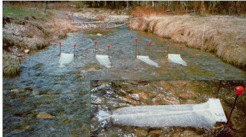
Figure 8: Bedload traps in Little Granite Creek, with bedload trap detail.
