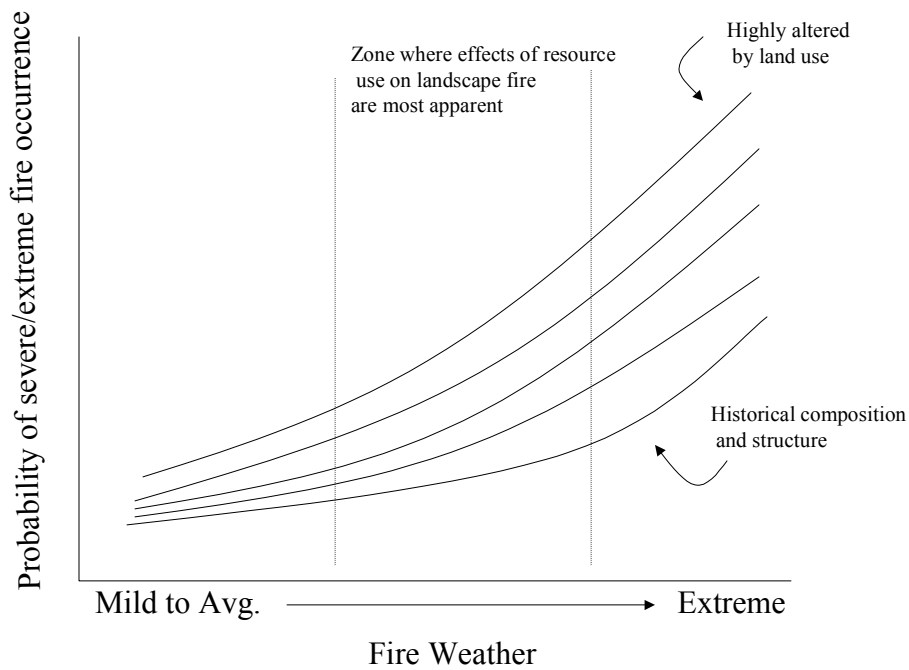
Figure 1. Conceptual relationships of how land and water affects fire behavior and severity along a gradient of increasing fire weather conditions (temperature, relative humidity, wind speed, fuel moisture content).
