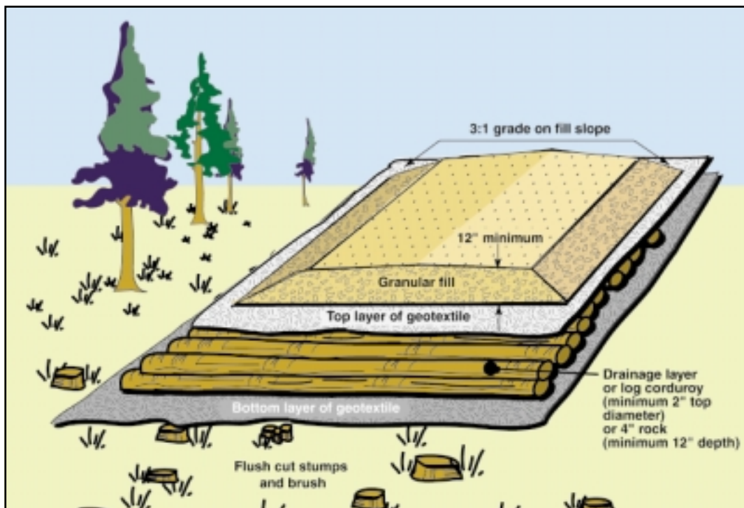
Figure 8—Road design for peat wetlands with continuous cross drainage. Drainage layers may be used as an alternative to culverts, or in combination with culverts, to provide adequate cross drainage.
