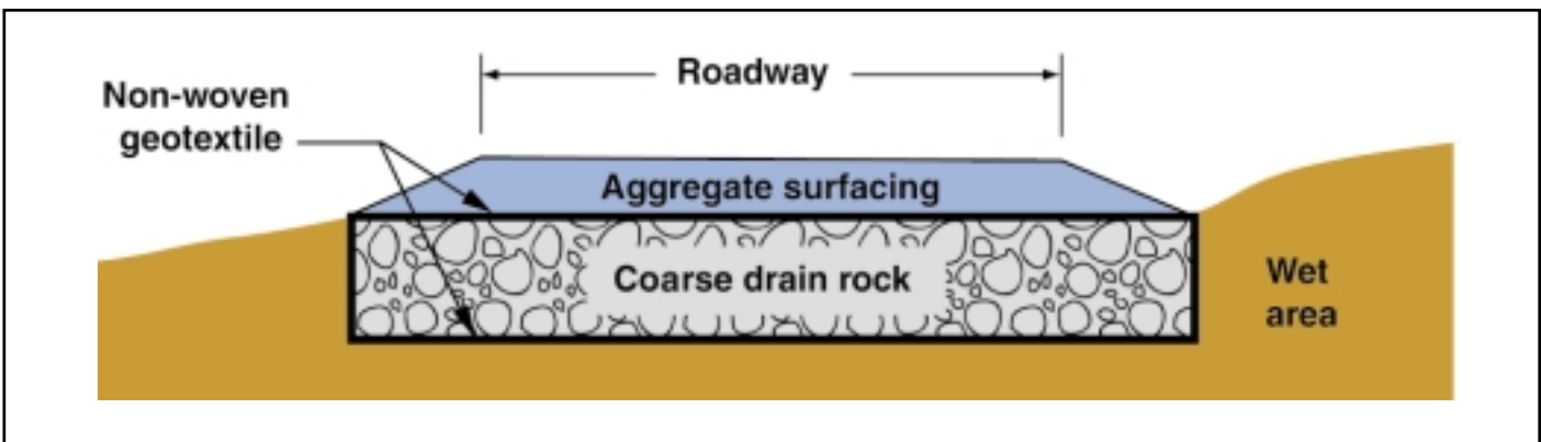
Figure 14—French drain. Not to scale.
