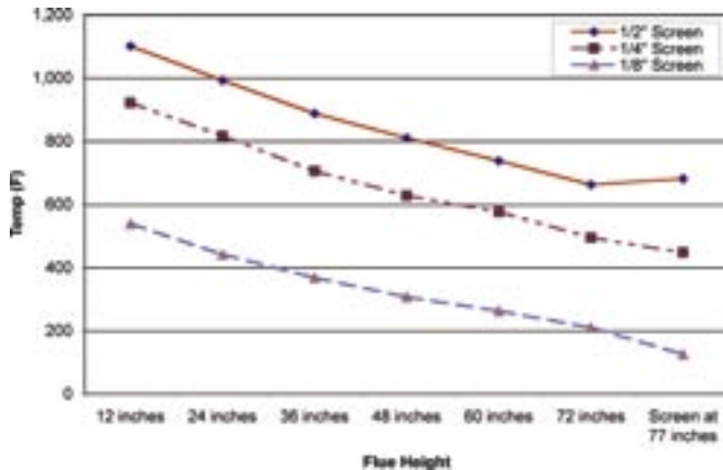
Figure 2. Flue height versus average flue center temperature.
