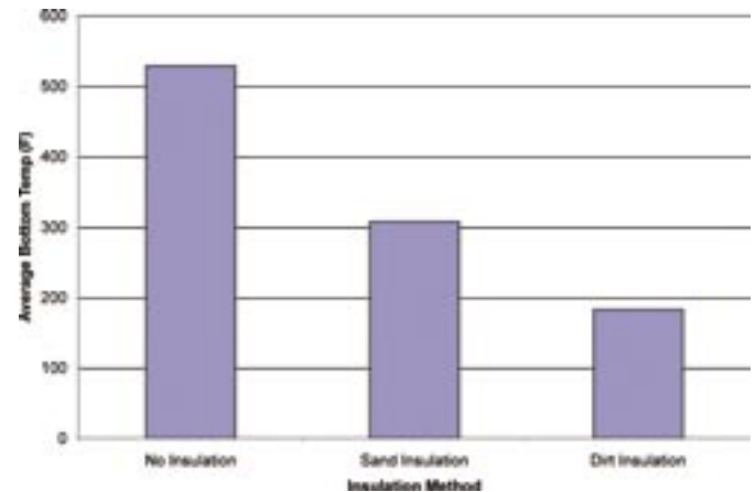
Figure 3. Average stove bottom temperature versus insulation method.
