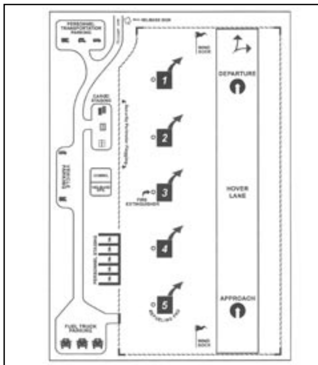
Figure 5—Helibase layout.
