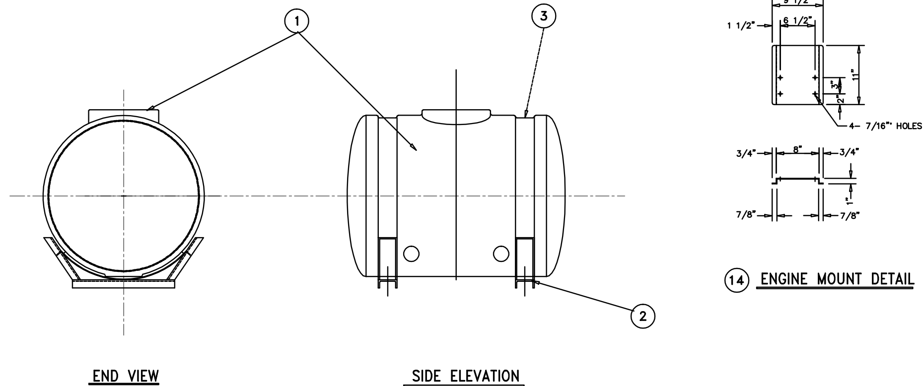
TANK AND CRADDLE
