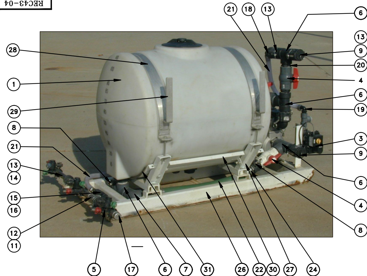
TANK, CRADLE & ROLL OFF MODULE
