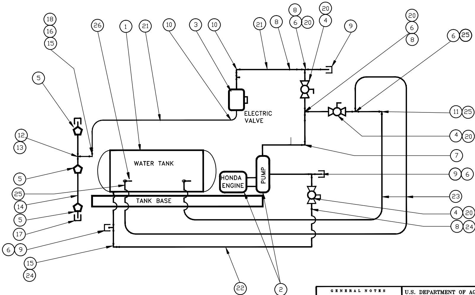
FLOW DIAGRAM
