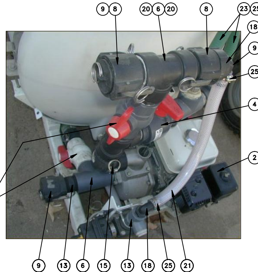
FRONT OF TANK
