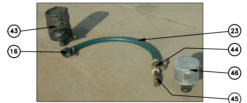
TANK ACCESSORIES
