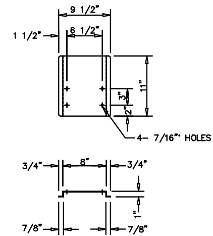
14 ENGINE MOUNT DETAIL
