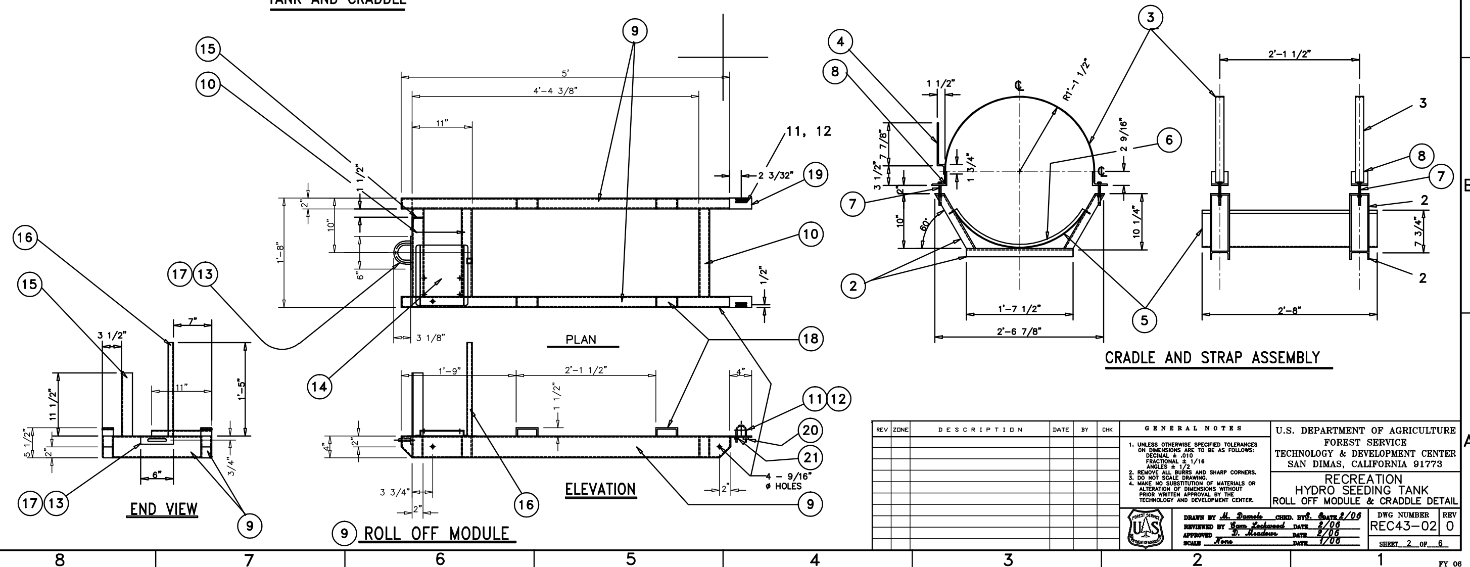
TANK AND CRADDLE
