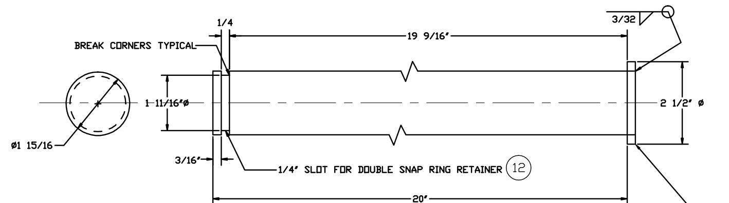
10 LIFT PIVOT PIN
