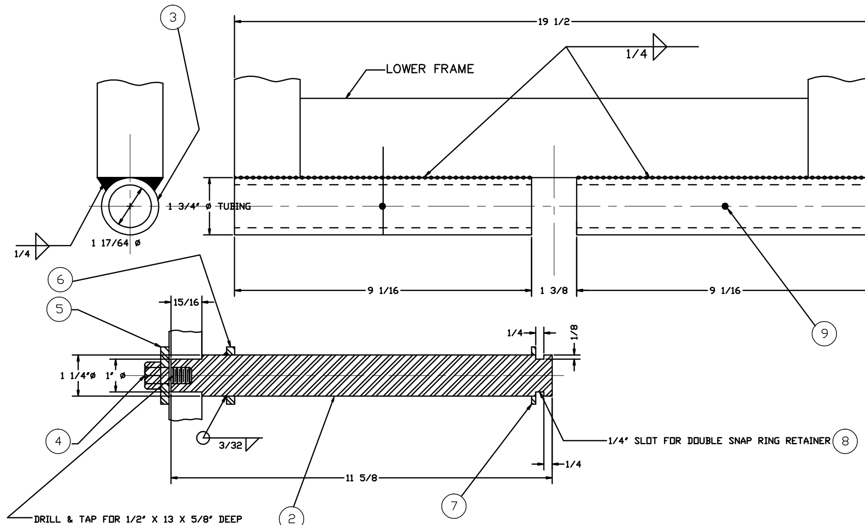
1 WALKING BEAM AXLE ASSEMBLY
