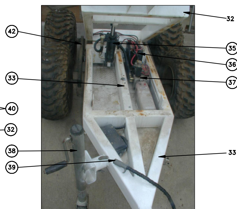
TRAILER LOWER FRAME
