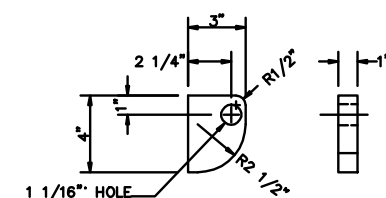
⑤ HYDRO LIFT BRACKET
