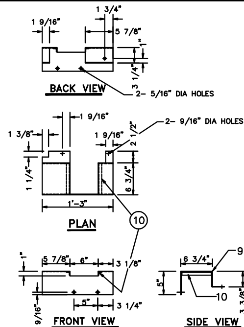
⑨ WINCH COVER
