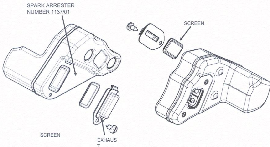
SIDE MUFFLER WITH SIDE- DOWNWARD EXHAUST OUTLET
