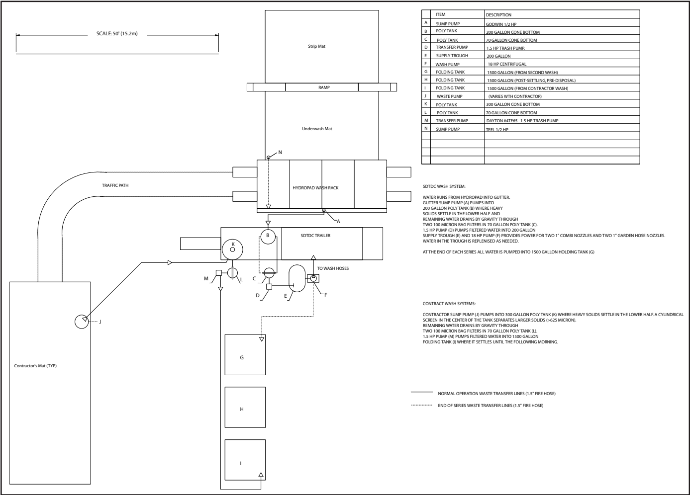
Figure 8—Waste-recovery drawing.
