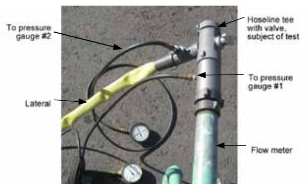
Figure 2—Sample setup of hoseline tee test.
