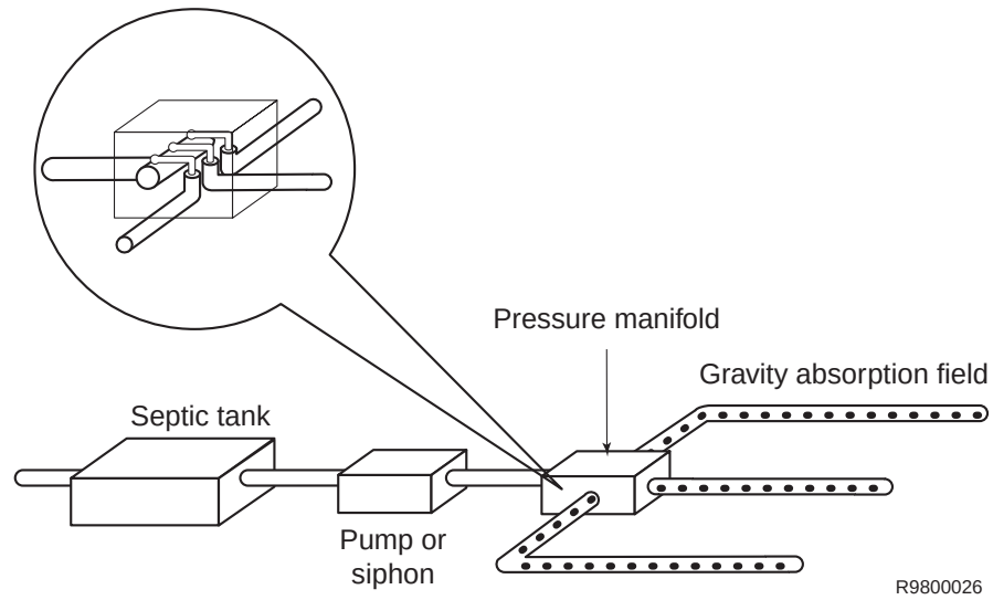
Figure 19—Diagram of a pressure dosed distribution system.
