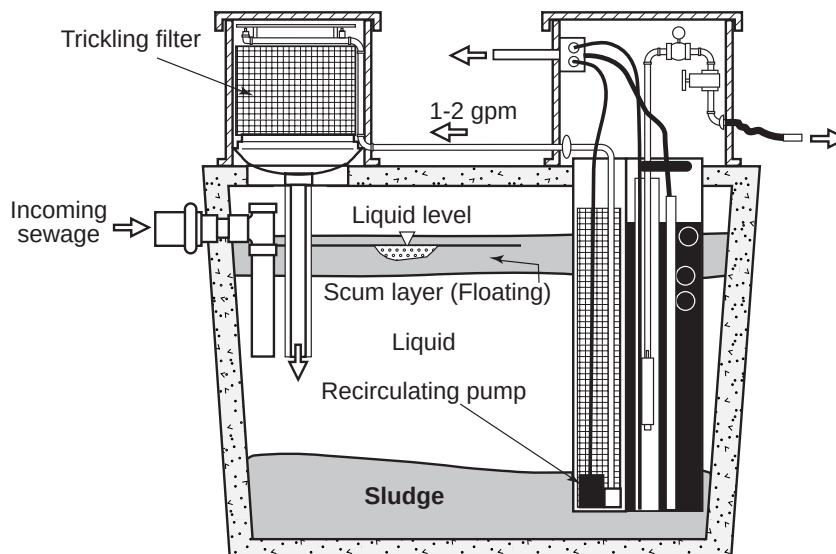
Figure 13—Recirculating trickling filter schematic.
