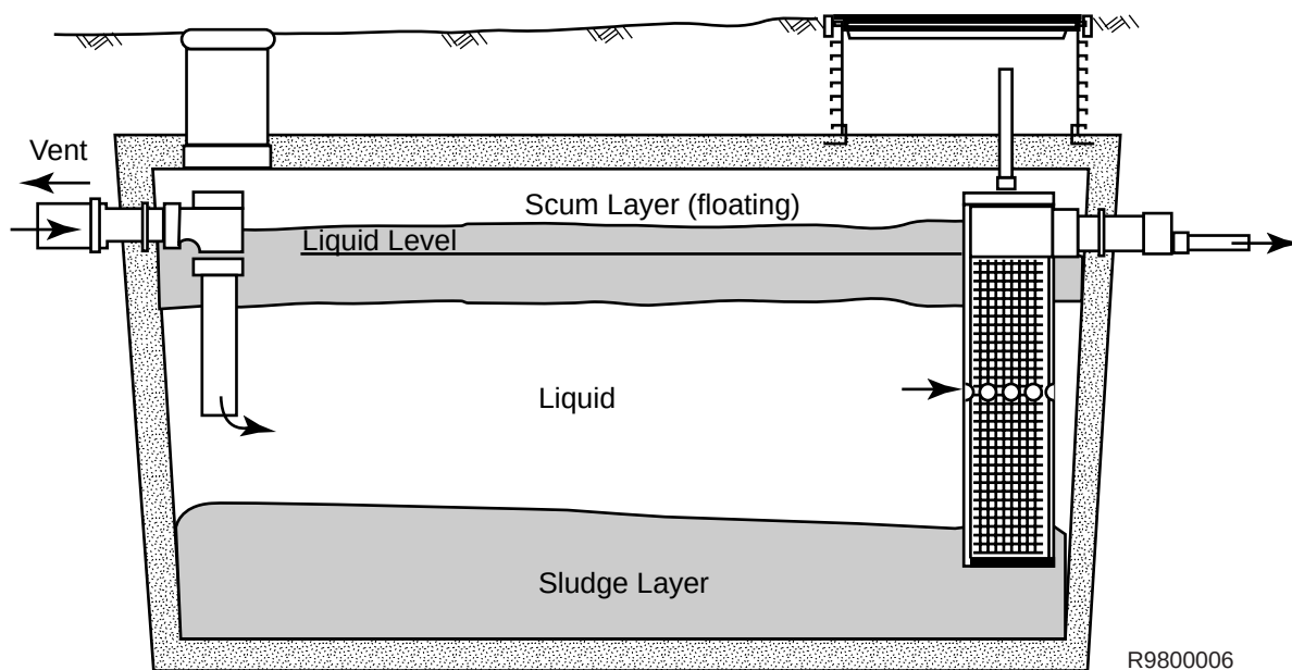
Figure 1—Diagram of a septic tank filter.
