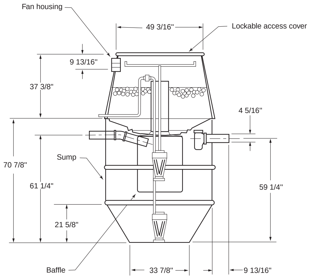
Figure 10—Bioclere schematic.
