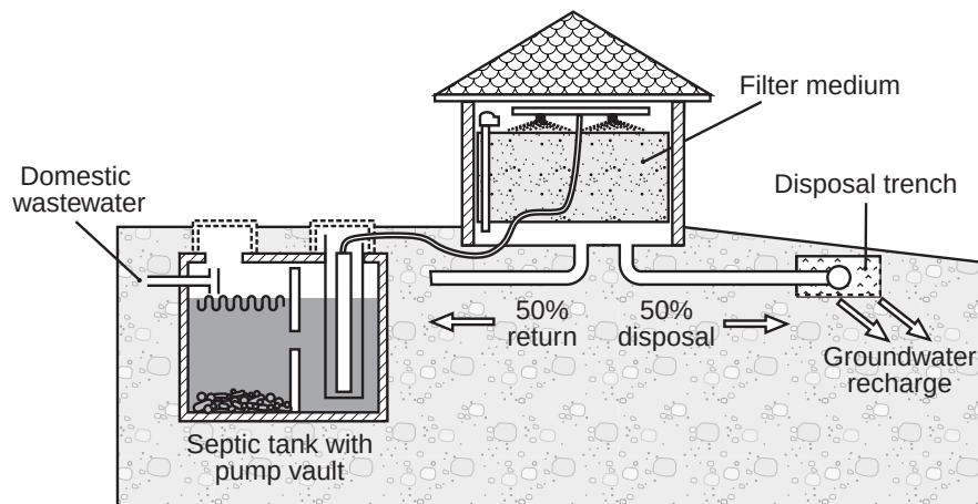
Figure 2—Diagram of the Waterloo Biofilter.
