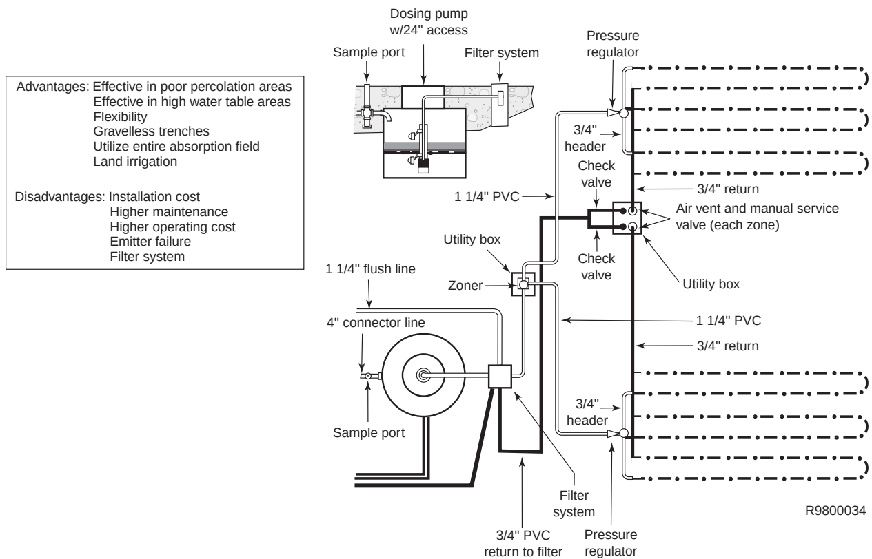
Figure 27—Emitter system.
