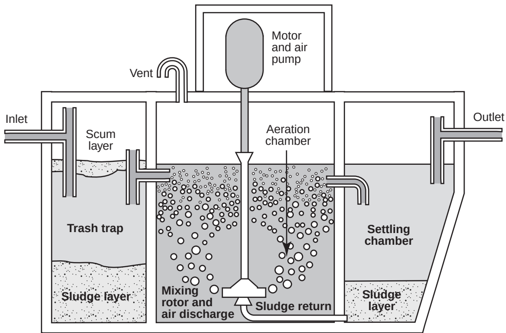
Figure 4—Diagram of an aerobic system.
