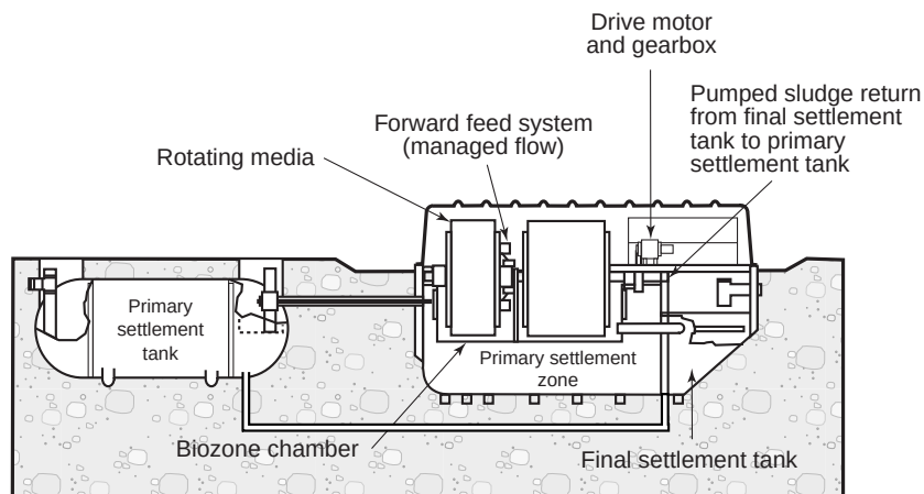
Figure 5—RBC system.
