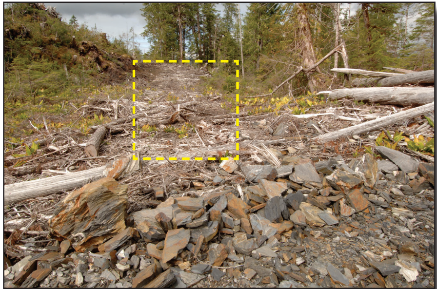
Figure 4-38—Vegetation: Sitka spruce and western hemlock. Surface soil texture is a gravelly silt loam. A shovel-yarding technique is used on slopes less than 20 percent. Slash mats are constructed to prevent rutting and support the weight of the shovel yarder (excavator). The soils have low bearing strength and adverse soil effects are avoided by combining a slash mat and equipment with a low (7 to 10 pounds per square inch) static load. Ecomap Section M245C - Southern Alexander Archipelago, Tongass National Forest, Alaska Region.
