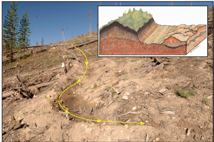
Figure 2-7—Displaced soil creates a berm along the skid trail by moving the topsoil (A horizon).
