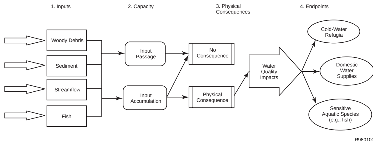
Figure 2—Road-stream crossing and cross drain environmental risk can be expressed as a four part model consisting of inputs—those materials delivered to the culvert; capacity—the ability of the structure to maintain the natural transport regime of the delivered inputs; physical consequences—the erosional and/or depositional consequences occurring when capacity is exceeded; and endpoints—potentially affected aquatic and riparian resources, human uses, and other values.
