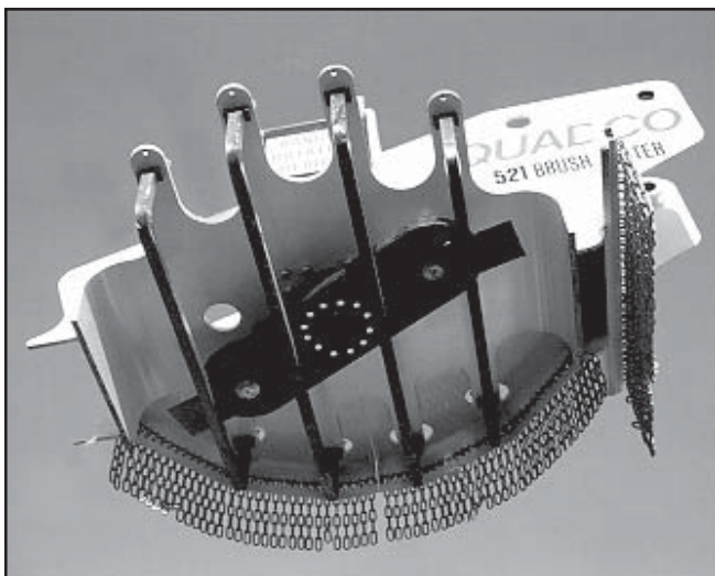
Figure 7—The Brushco brush-cutter attachment (made by Quadco) for excavators.
