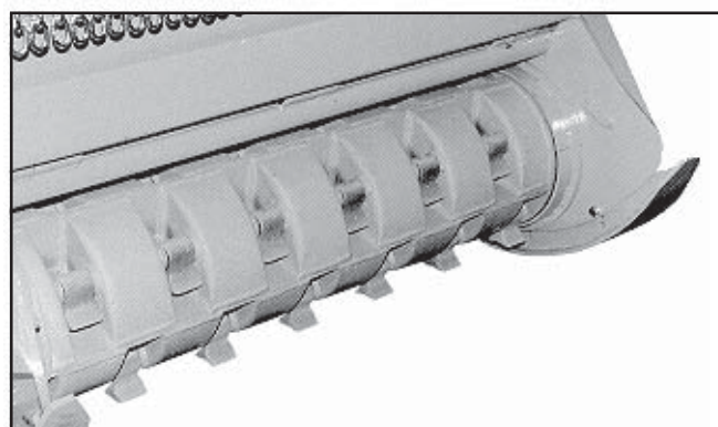
Figure 4—Seppi M drum shredder with free-swinging cutters.
