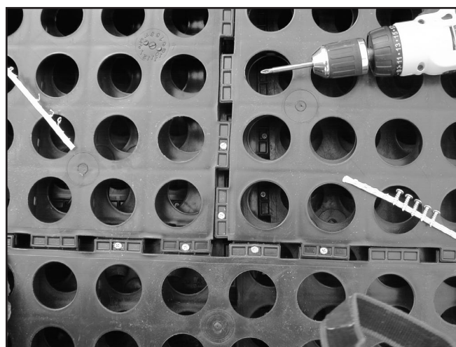
Figure B3—Illustration of the tab-fastening screw pattern at panel joints.
