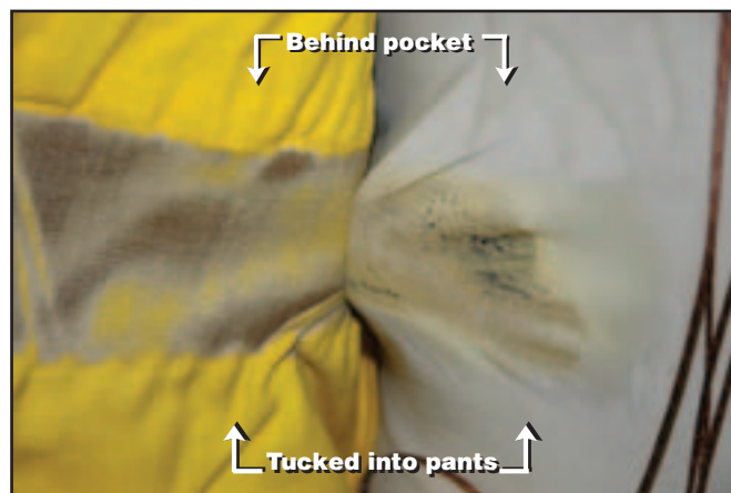
Figures 6b—A significant, but smaller, portion of the Under Armour undershirt (off white) melted during the test. The portions of the undershirt that were behind the shirt pocket and tucked into the pants did not melt.
