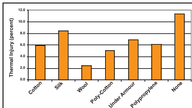
Figure 5—The percentage of the mannequin that would be predicted to have second-degree or more serious burns for each type of undershirt.
