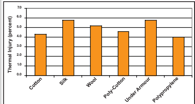
Figure 9—The percentage of the back of the mannequin estimated to have second-degree thermal injury with each type of undergarment. The back represents 10.8 percent of the entire body.
