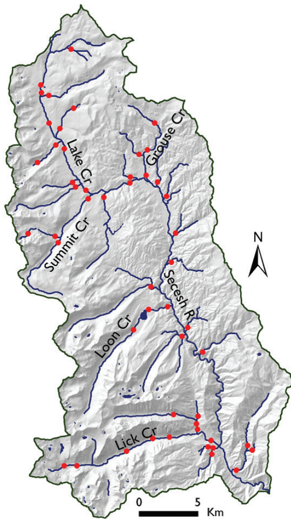
Figure 12. Distribution of thermographs in 2006. Locations were selected to encompass a range of elevations and contributing areas.
