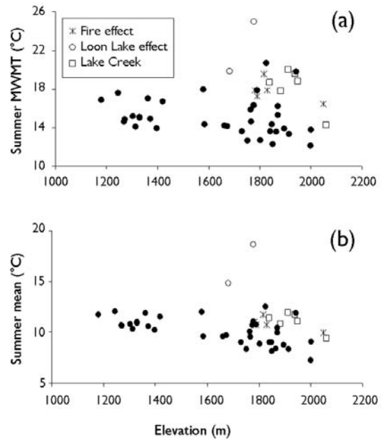
Figure A3. Scatterplots of stream temperature versus elevation within the Secesh River Watershed for summer: (a) MWWT and (b) mean.
