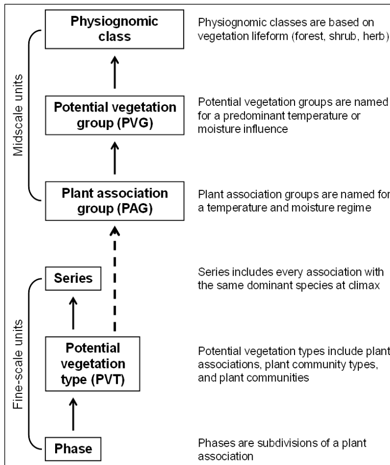
Figure 1-3 – Potential vegetation (PV) hierarchy for the Blue Mountains (from Powell et al. 2007). PV taxonomic units have been organized as two integrated portions of a hierarchy. Fine-scale hierarchical units are described in PV classification reports (Crowe and Clausnitzer 1997, Johnson 2004, Johnson and Clausnitzer 1992, Johnson and Simon 1987, Johnson and Swanson 2005, Swanson et al. 2010, and Wells 2006); midscale units are primarily described in reports from an Interior Columbia Basin Ecosystem Management Project (such as Jensen et al. 1997). Potential vegetation types (PVTs) provide a link between the fine- and mid-scale portions of the hierarchy because PVTs are aggregated to form plant association groups. Stocking level and stand density information was developed for PAGs and PVGs by generalizing PVT-level data (Powell 2013b).
