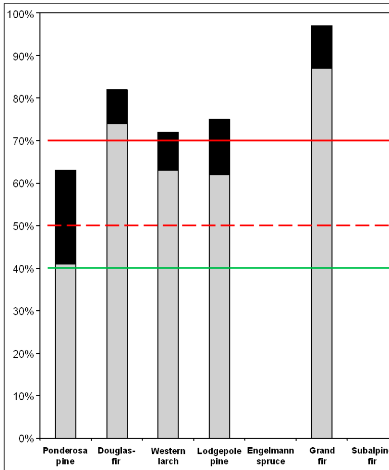
Figure 4-9 – Canopy cover estimates for tree species of the Dry Upland Forest potential vegetation group (from Powell 2012). Blue Mountain elk cover standards (Thomas et al. 1979) use canopy cover limits: satisfactory cover is \geq 70\% cover (solid red line), and marginal cover is \geq 40\% canopy cover (solid green line). Bars are canopy cover estimates calculated by using Dealy's (1985) equations to convert basal area to canopy cover. The black portion of each bar shows canopy cover in the self-thinning zone (above the upper limit of a management zone, ULMZ); gray portion shows canopy cover below the ULMZ (cover values taken from Powell 2013b). The Umatilla NF Forest Plan (USDA Forest Service 1990) has a separate satisfactory cover threshold for ponderosa pine (50% canopy cover), and it is shown here with a dashed red line. For the 70% satisfactory cover threshold, only dry-forest stands with a predominance of Douglas-fir or grand fir could provide that much canopy cover and still remain below the self-thinning zone.
