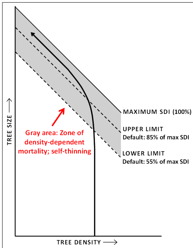
Figure 4-1 – Forest Vegetation Simulator (FVS) stocking level system. This section of chapter 4 covers each parameter shown in this diagram: maximum SDI, upper limit, and lower limit, and it describes how users can modify them by using the SDIMAX keyword. Note: ‘Upper Limit’ and ‘Lower Limit’ in this diagram do NOT refer to the upper and lower limits of a management zone, which are described in chapter 3.
