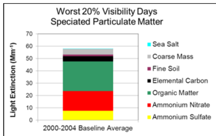
Figure 13. Composition of Particulate Matter on the Hazeiest Days at the Eagle Cap and Strawberry Mountain Wilderness Areas.
