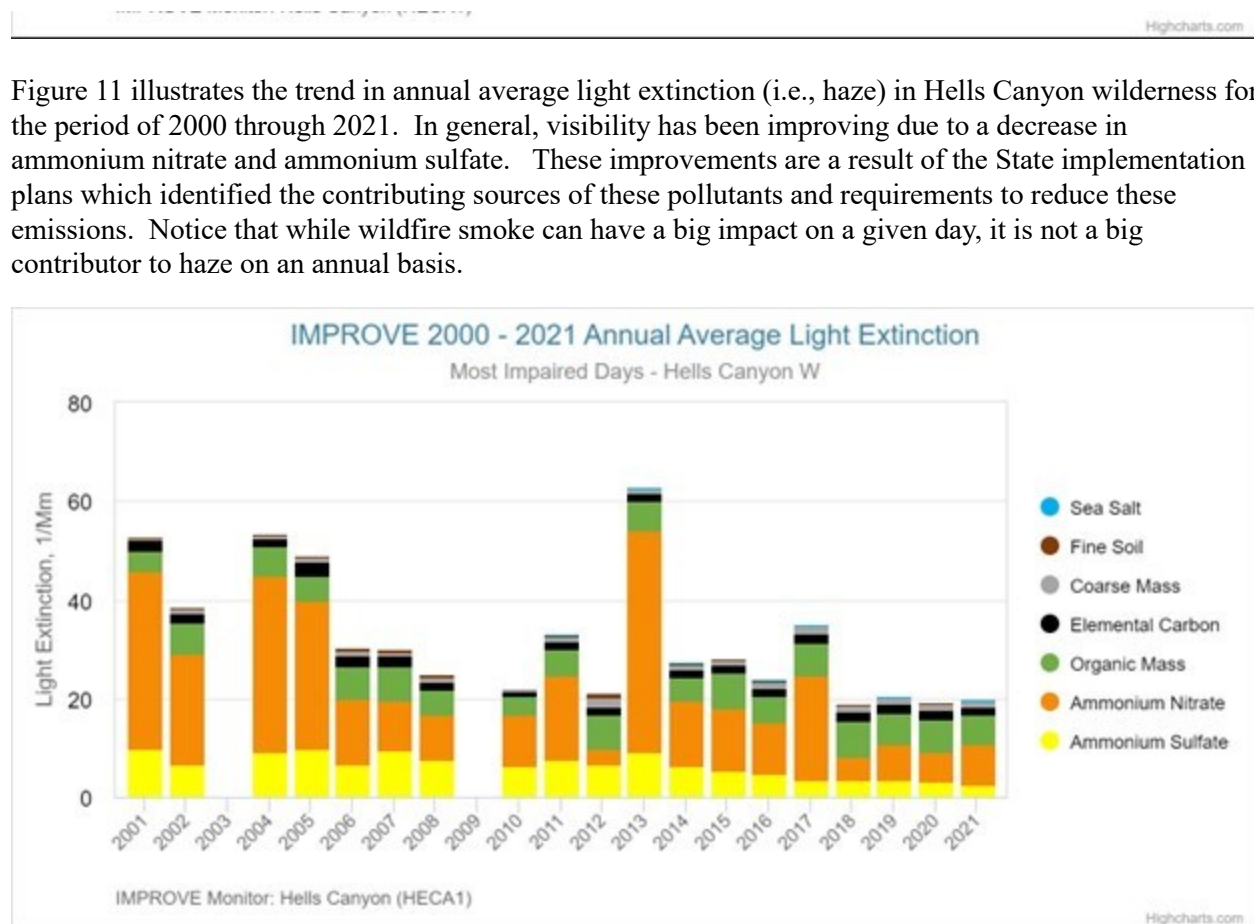
Figure 11. Visibility Trends and Future Projections in Hells Canyon Wilderness
