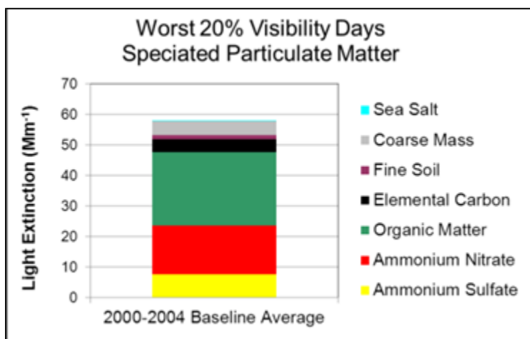
Figure 13 illustrates the primary pollutants which are causing the haze in the Eagle Cap and Strawberry Mountain Wilderness areas during the worst 20% days. Organic matter, ammonium nitrate and ammonium sulfate are the largest contributing pollutants to haze.
