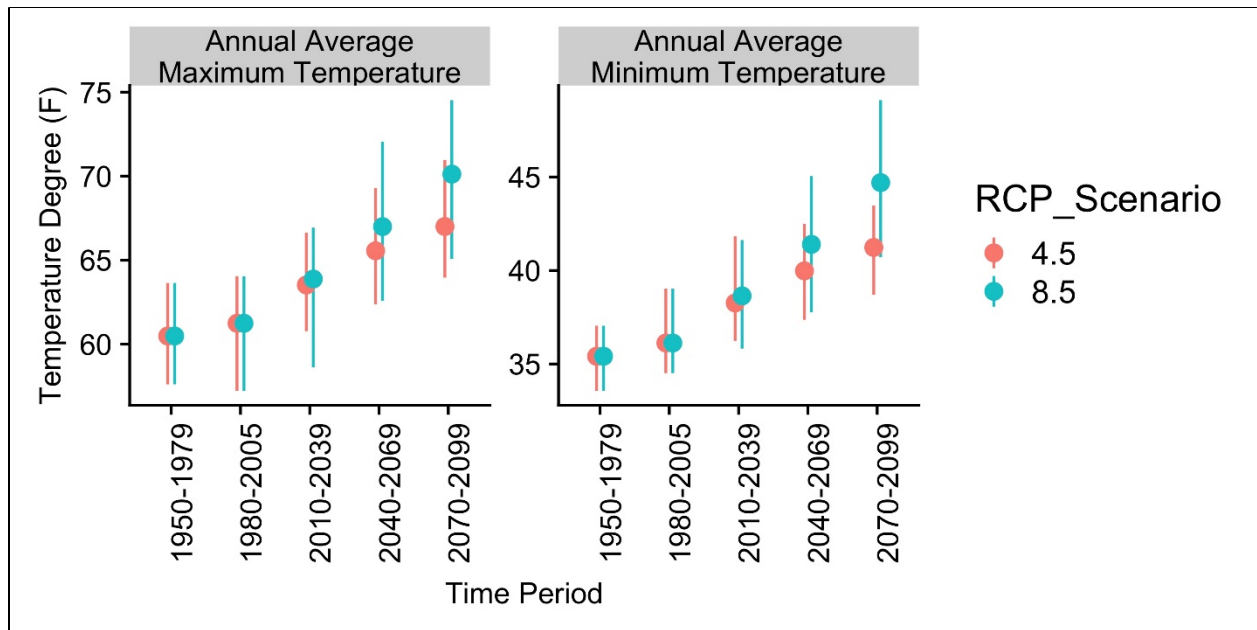
Figure 12. Modeled historic and future average minimum and maximum temperature on the Eldorado National Forest summarized for 30-year periods. Points represent average while lines indicate range of data (minimum and maximum). Data source CalAdapt: See Table 4 footnote.
