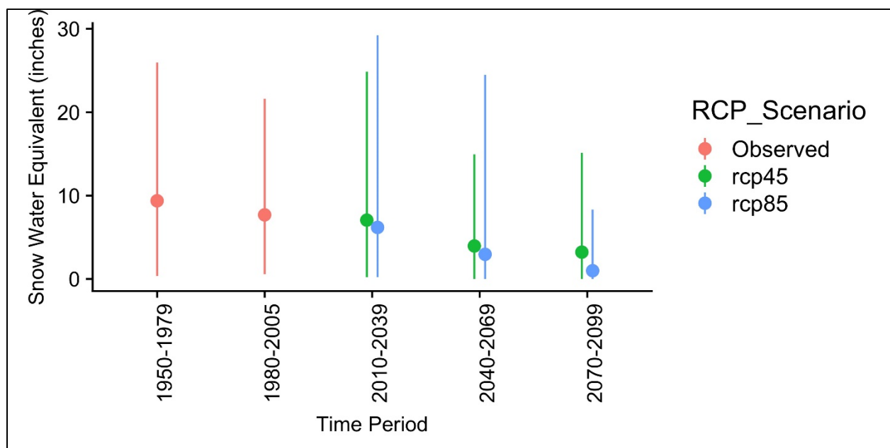
Figure 18: Historic observed and future predicted April 1 st Snow Water Equivalent (SWE) on the Eldorado National Forest summarized for 30-year periods under two emission scenarios (RCP 4.5 and RCP 8.5). Points represent average while lines indicate range of data (minimum and maximum). Data source CalAdapt: See Table 4 footnote.
