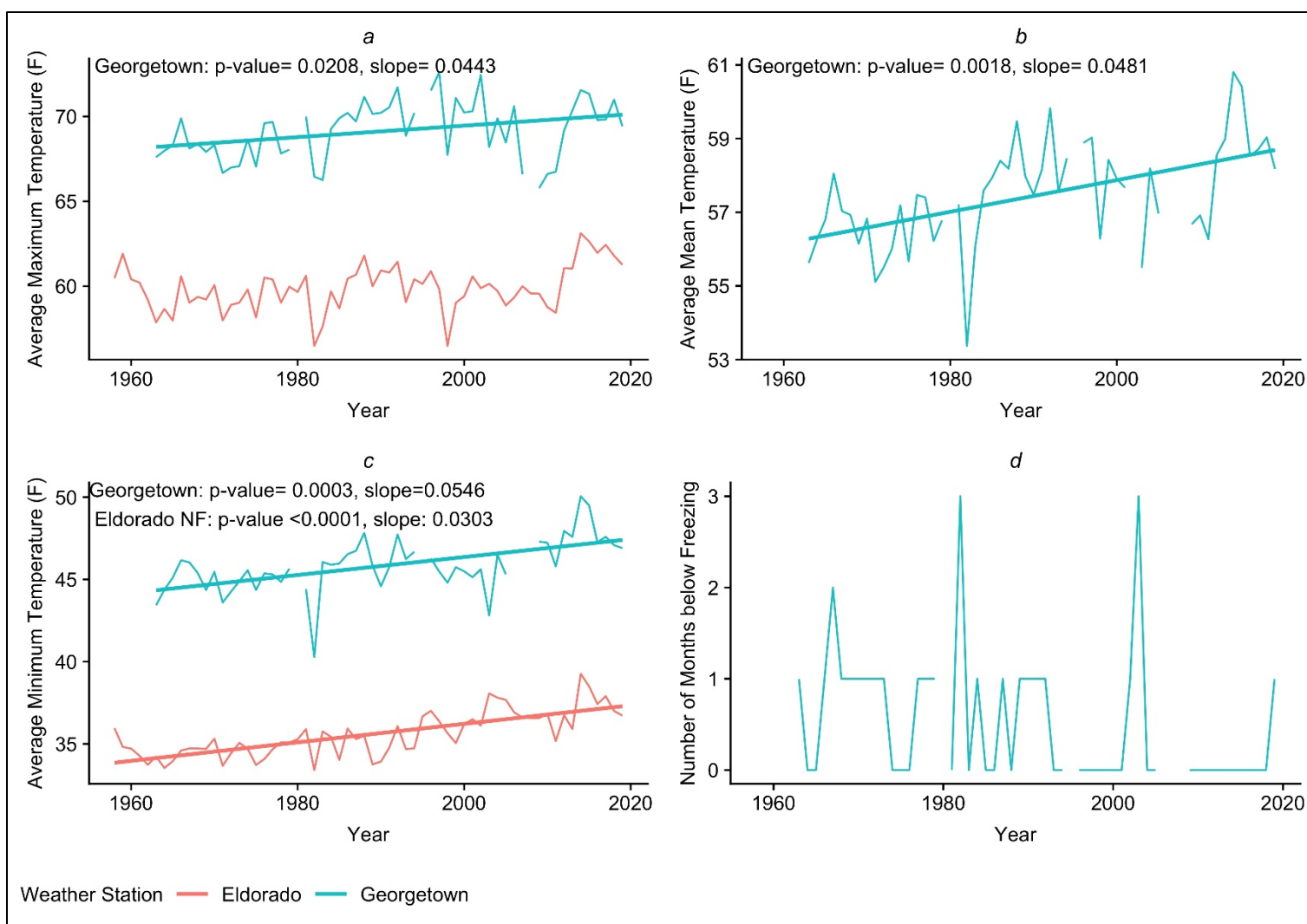
Figure 2. Historic temperature trends for Eldorado National Forest weather stations (identified in different colors): a) Average Maximum Temperature, b) Average Mean Temperature, c) Average Minimum Temperature, and D) Number of Months below Freezing (months where the average minimum temperature was <32°F). Linear lines indicate a significant trend. For all significant trends the level of significance (p-value) and magnitude and direction of trend (slope) are presented.
