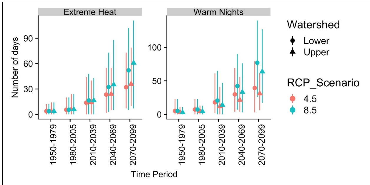
Figure 14. Modeled extreme heat days and warm nights for the Upper North Fork Mokelumne Watershed and the Rock Creek Watershed on the Eldorado National Forest summarized for 30-year periods. Points represent the average while lines indicate range of data. Data is based on the 98 th percentile for what is currently considered extremely hot for the specific area between April through October. The 98 th percentile for extreme heat (maximum temperature) is 81°F and 103.2°F and for warm nights (minimum temperature) is 51°F and 66.4°F for the Upper North Fork Mokelumne Watershed and the Rock Creek Watershed, respectively. Data source CalAdapt: See Table 4 footnote.
