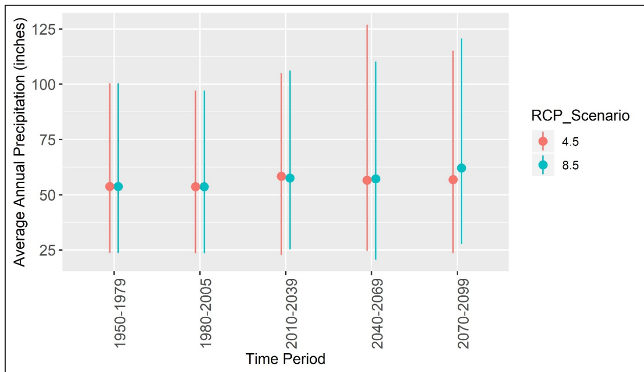
Figure 15. Modeled historic and future average annual precipitation on the Eldorado National Forest summarized for 30-year periods. Points represent average while lines indicate range of data (minimum and maximum). Data source CalAdapt: See Table 4 footnote.
