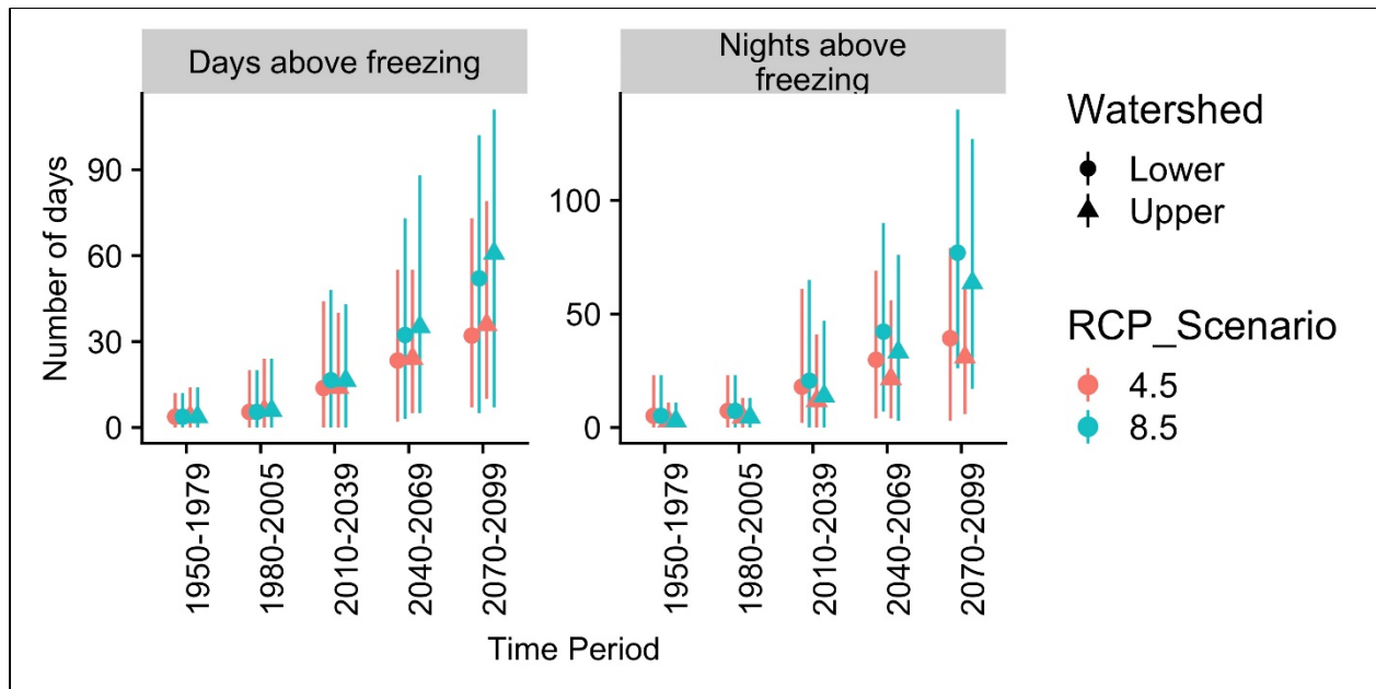
Figure 13. Modeled number of days above freezing (32°F) for the Upper North Fork Mokelumne Watershed and Rock Creek Watershed on the Eldorado National Forest summarized for 30-year periods. Points represent the average while lines indicate range of data. Data source CalAdapt: See Table 4 footnote. Days above freezing and nights above freezing are based on when the daily maximum/minimum exceeds 32°F.
