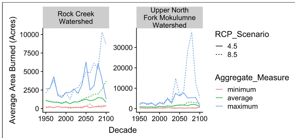
Figure 22. Wildfire simulations for two watersheds on the Eldorado National Forest smoothed by decade. Data source CalAdapt using wildfire scenario projections produced by (Westerling 2018).
