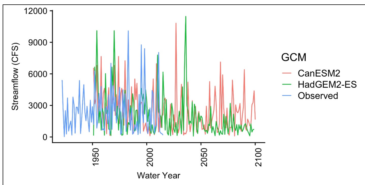
Figure 20. This chart shows total annual unimpaired flows in a water year (October – September) for June, July, and August. Data are shown Mokelumne River at Pardee Reservoir under the RCP 8.5 scenario in which emissions continue to rise strongly through 2050 and plateau around 2100. Values represent observed streamflow (1922-2015) and global climate models (GCM) of CanESM2 (an average simulation) and HadGEM2-ES (a warm/drier simulation).
