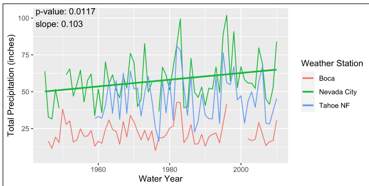
Figure 3. Total precipitation for local weather stations (identified in different colors).
