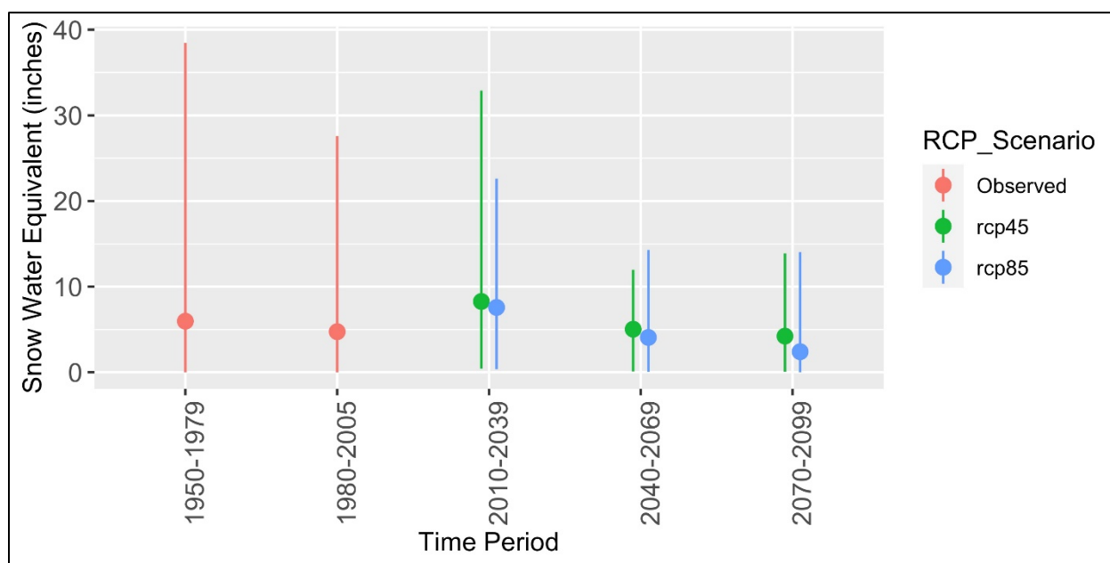
Figure 18: Historic observed and future predicted April 1 st Snow Water Equivalent (SWE) on the Tahoe National Forest summarized for 30-year periods under two emission scenarios (RCP 4.5 and RCP 8.5).
