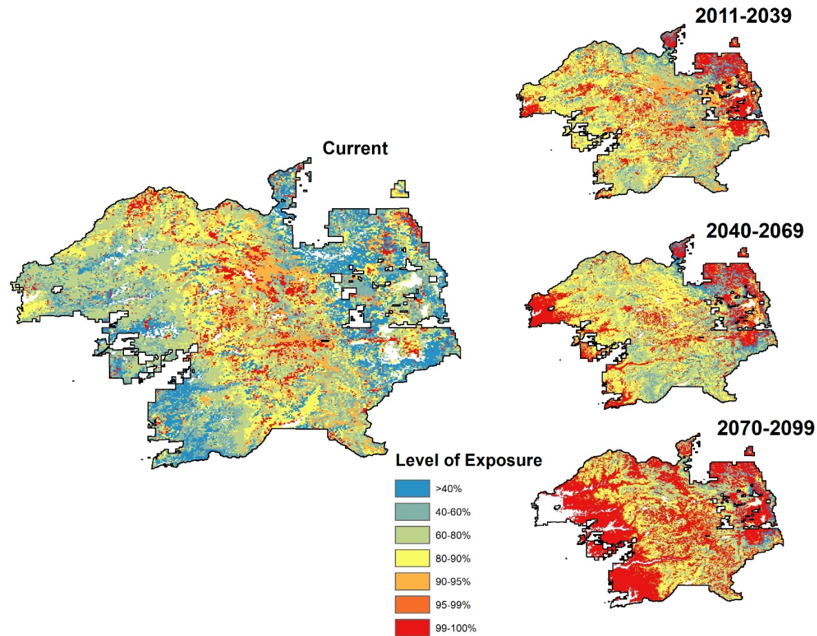
Figure 23. Mapped climate exposure under the “Warm and Wet” CNRM CM5 climate projection under Higher Emissions RCP8.5. This image shows the climate exposure of vegetation types at current time and three future periods: 2011–2039, 2040–2069, and 2070–2099. Areas considered to be highly climatically exposed are in the 95–99% and 99–100%. Areas with values <80% are considered to be in climatically suitable conditions for the vegetation that it currently occupies.
