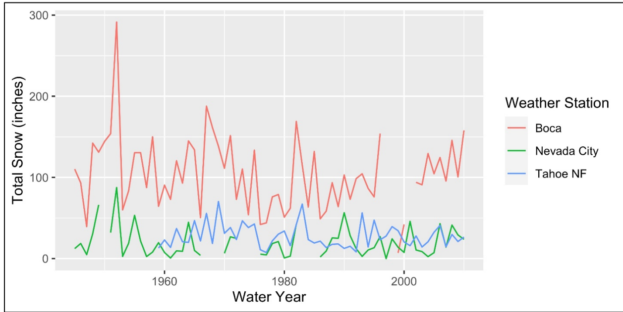
Figure 4. Total snowfall for local weather stations (identified in different colors). Linear lines indicate a significant trend. For all significant trends the level of significance (p-value) and magnitude and direction of trend (slope) are presented. *Note that data for the Tahoe National Forest (Terra Climate) are Snow Water Equivalent (in inches), while data for the individual weather stations are Total Snow (in inches).
