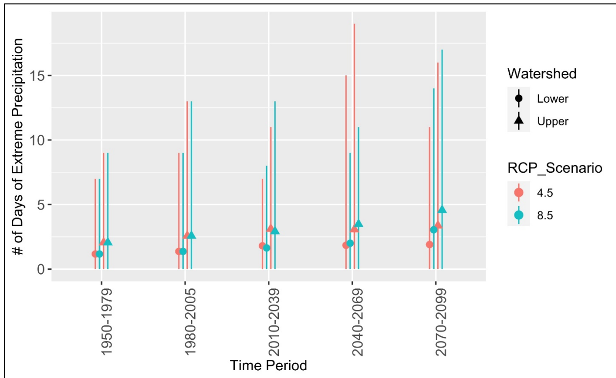
Figure 16. Modeled number of days of extreme precipitation in a water year with 2-day rainfall totals above the extreme threshold for the Little Truckee River Watershed (3.38 inches) and the Lower Middle Fork American River Watershed (2.99 inches) on the Tahoe National Forest summarized for 30-year periods. Points represent average, while lines indicate the minimum and maximum. Data source CalAdapt: See Table 4 footnote.
