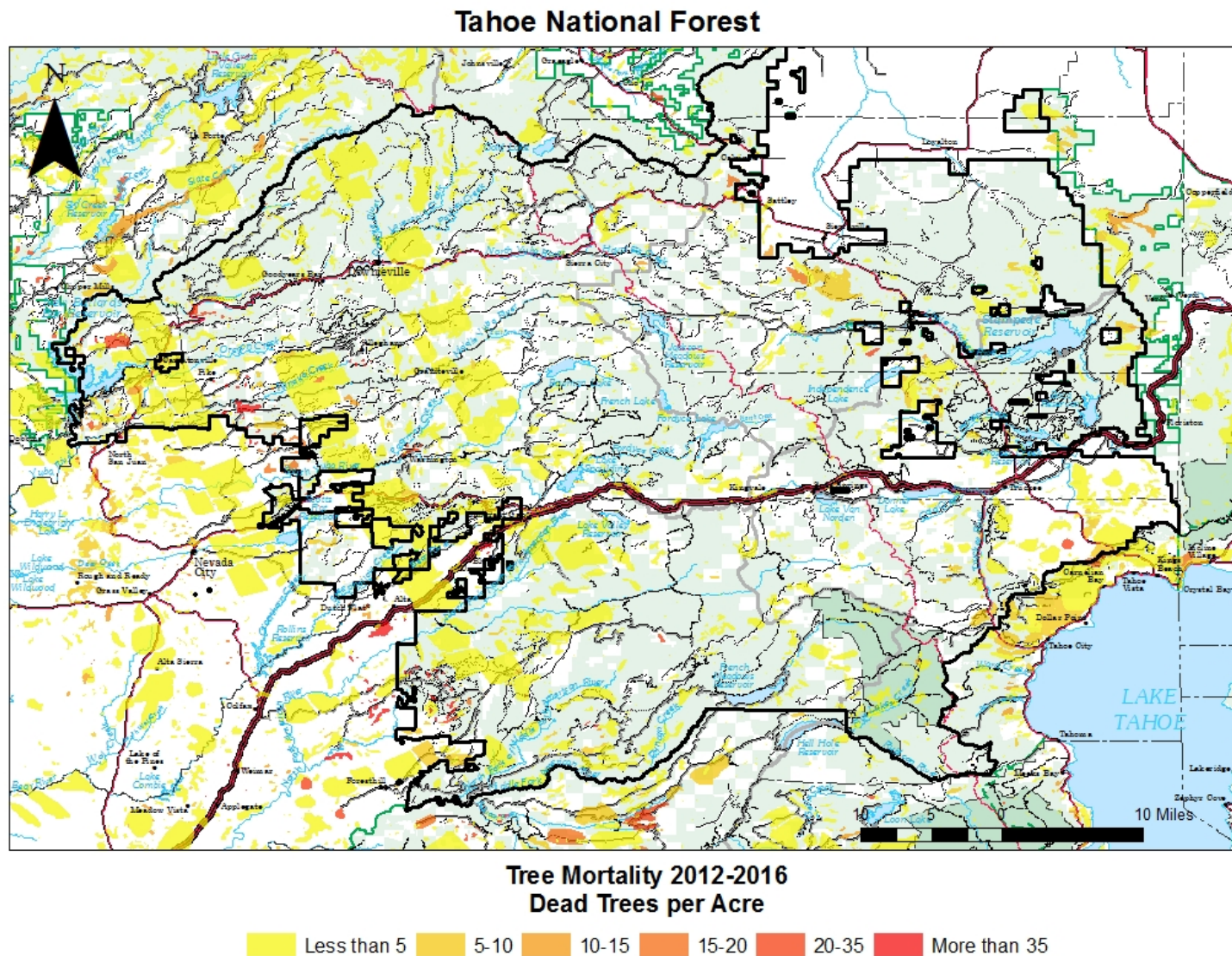
Figure 9. Recent (2012-2016) cumulative drought and insect-related mortality in the Tahoe National Forest based on aerial detection surveys by the drought. Forest Service Forest Health Protection.
