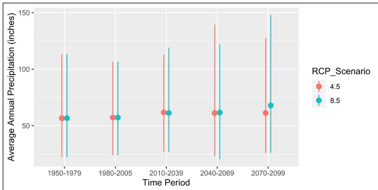
Figure 15. Modeled historic and future average annual precipitation on the Tahoe National Forest summarized for 30-year periods. Points represent average while lines indicate range of data (minimum and maximum). Data source CalAdapt: See Table 4 footnote.
