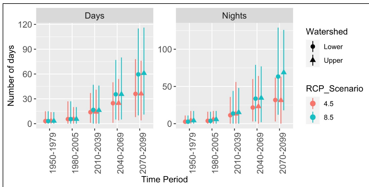
Figure 14. Modeled extreme heat days and warm nights for the Little Truckee River Watershed and the Lower Middle Fork American River Watershed on the Tahoe National Forest summarized for 30-year periods. Points represent the average while lines indicate range of data. Data is based on the 98 th percentile for what is currently considered extremely hot for the specific area between April through October. The 98 th percentile for extreme heat (maximum temperature) is 86.3 and 98.8°F and for warm nights (minimum temperature) is 45.2 and 69.4°F for the Little Truckee River Watershed and the Lower Middle Fork American River Watershed respectively. Data source CalAdapt: See Table 4 footnote.
