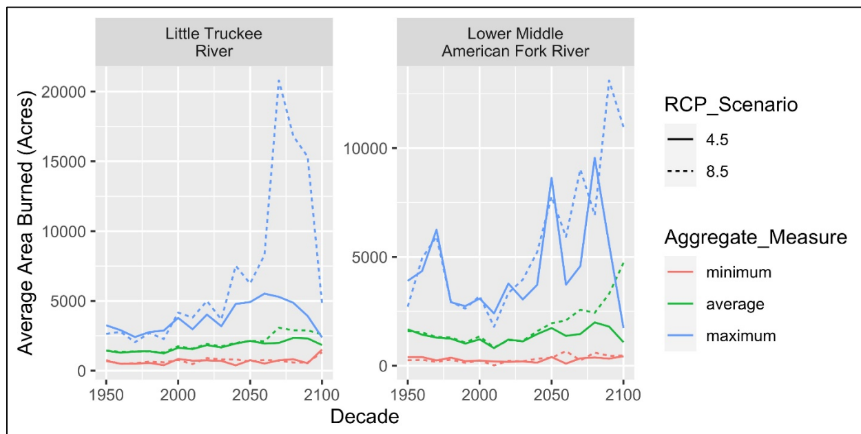
Figure 22. Wildfire simulations for two watersheds on the Tahoe National Forest smoothed by decade. Data source CalAdapt using wildfire scenario projections produced by (Westerling 2018).
