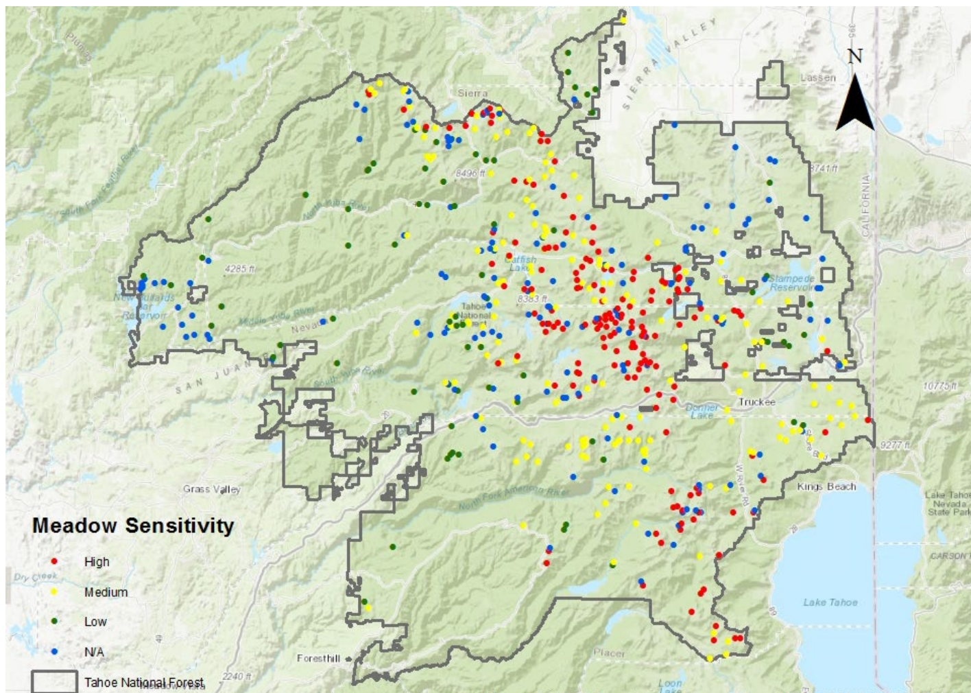
Figure 10. Meadow sensitivity on the Tahoe National Forest based on the slope of the relationship between April 1st snowpack and late season greenness (Normalized Difference Vegetation Index-NDVI) between 1984 to 2016.
