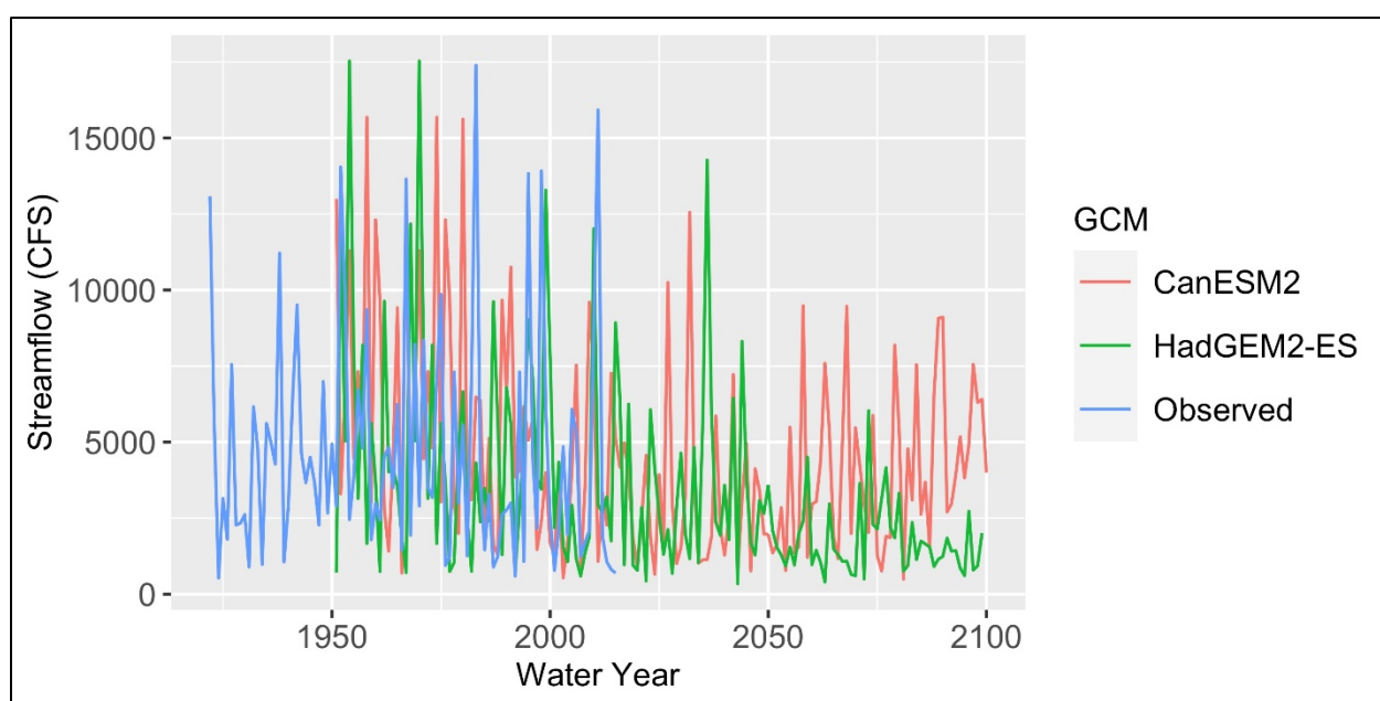
Figure 20. This chart shows total annual unimpaired flows in a water year (October – September) for June, July, and August. Data are shown for Yuba River at Smartville under the RCP 8.5 scenario in which emissions continue to rise strongly through 2050 and plateau around 2100. Values represent observed streamflow (1922-2015) and global climate models (GCM) of CanESM2 (an average simulation) and HadGEM2-ES (a warm/drier simulation).
