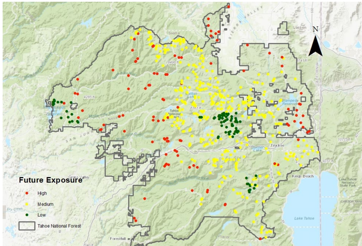
Figure 24. Future exposure of meadows on the based on the relative change in April 1 st snowpack between 1981-2010 and 2040-2069 using the climate model MIROC-RCP8.5.
