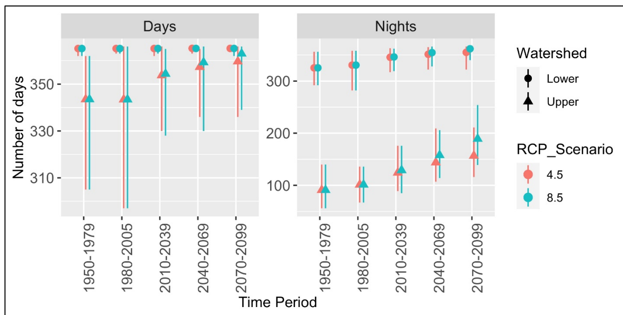
Figure 13. Modeled number of days above freezing (32°F) for the Little Truckee River Watershed and Lower Middle Fork American River Watershed on the Tahoe National Forest summarized for 30-year periods. Points represent the average while lines indicate range of data. Data source CalAdapt: See Table 4 footnote. Days above freezing and nights above freezing are based on when the daily maximum/minimum exceeds 32°F.
