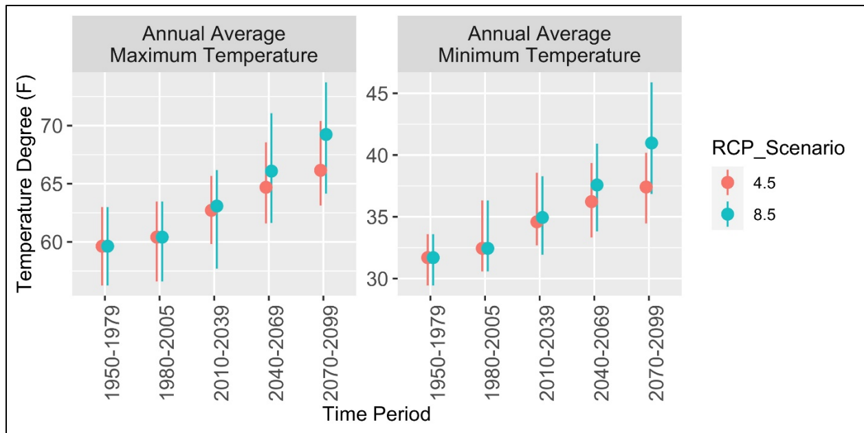
Figure 12. Modeled historic and future average minimum and maximum temperature on the Tahoe National Forest summarized for 30-year periods. Points represent average while lines indicate range of data (minimum and maximum). Data source CalAdapt: See Table 4 footnote.
