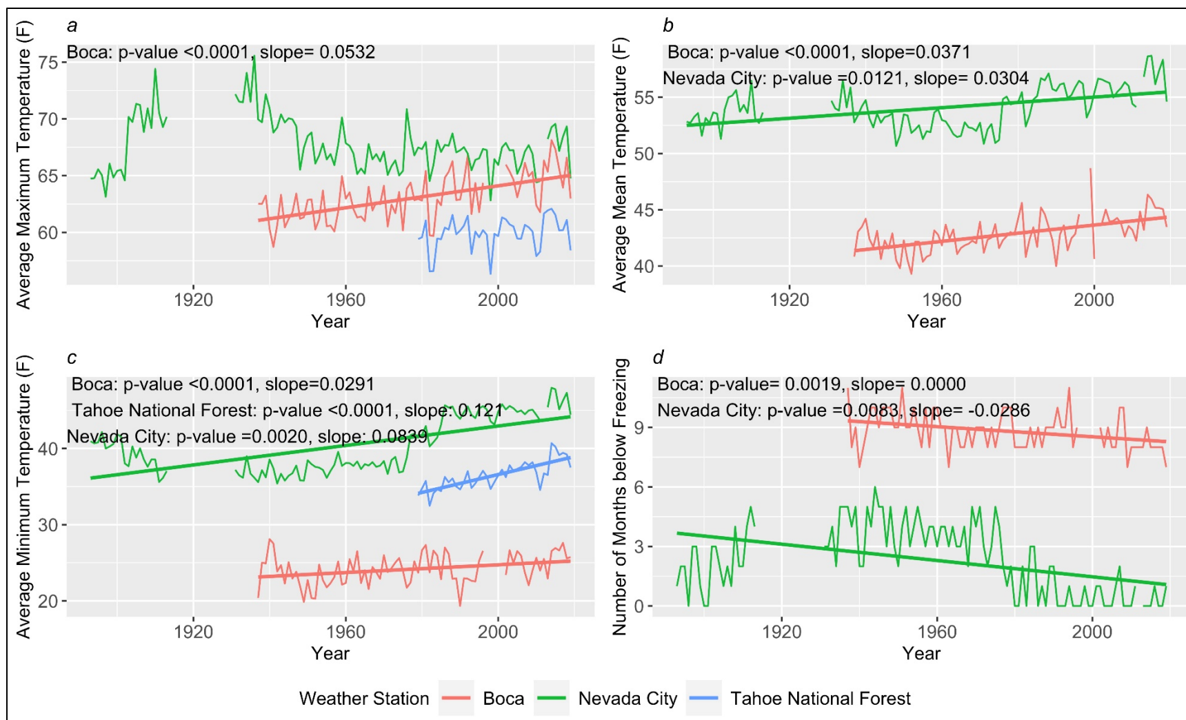
Figure 2. Historic temperature trends for weather stations (identified in different colors): a) Average Maximum Temperature, b) Average Mean Temperature, c) Average Minimum Temperature, and D) Number of Months below Freezing (months where the average minimum temperature was <32°F). Linear lines indicate a significant trend. For all significant trends the level of significance (p-value) and magnitude and direction of trend (slope) are presented.
