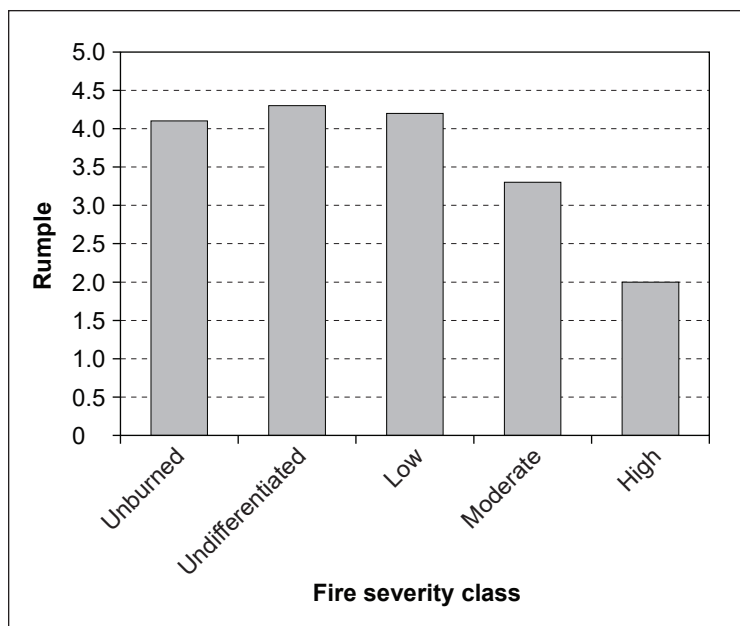
Figure 15—Mean rumple values for burned and unburned red fir forest landscapes of Yosemite National Park from Kane et al. (2013). Rumble is a measure of canopy surface rugosity and an indicator of canopy structural complexity and heterogeneity. All fire severity classes are statistically distinguishable ( P < 0.05 ) from each other.
