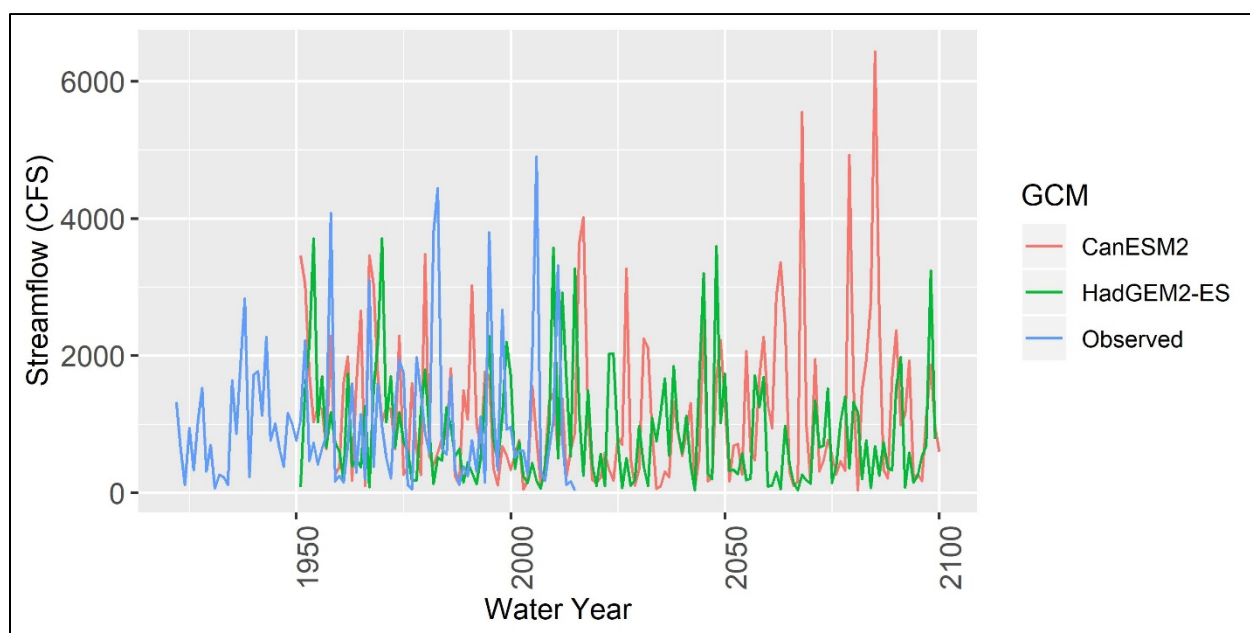
Figure 19. This chart shows total annual unimpaired flows in a water year (October – September) for June, July, and August. Data are shown for Calaveras River at Jeremy Lind under the RCP 8.5 scenario in which emissions continue to rise strongly through 2050 and plateau around 2100. Values represent observed streamflow (1922-2015) and global climate models (GCM) of CanESM2 (an average simulation) and HadGEM2-ES (a warm/drier simulation).
