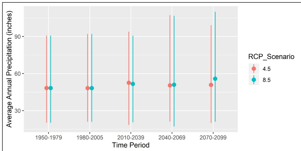
Figure 14. Modeled historic and future average annual precipitation on the Stanislaus National Forest summarized for 30-year periods. Points represent average while lines indicate range of data (minimum and maximum). Data source CalAdapt: See Table 4 footnote.
