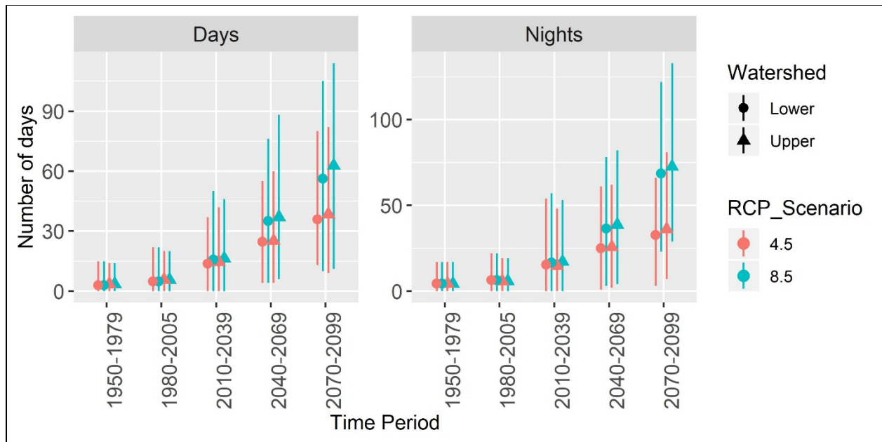
Figure 13. Modeled extreme heat days and warm nights for the Clark Fork Watershed and the Big Creek-Tuolumne River Watershed on the Stanislaus National Forest summarized for 30-year periods. Points represent the average while lines indicate range of data. Data is based on the 98 th percentile for what is currently considered extremely hot for the specific area between April through October. The 98 th percentile for extreme heat (maximum temperature) is 80.3°F and 97.0°F and for warm nights (minimum temperature) is 47.6°F and 61.7°F for the Clark Fork Watershed and the Big Creek-Tuolumne River Watershed, respectively. Data source CalAdapt: See Table 4 footnote.
