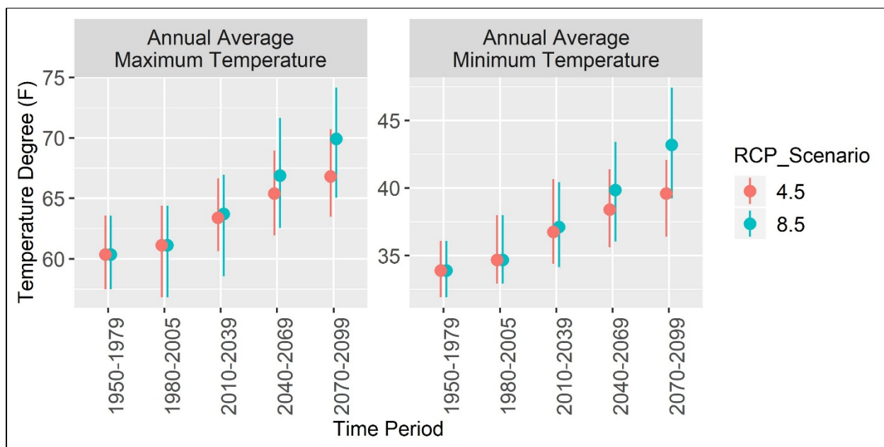
Figure 11. Modeled historic and future average minimum and maximum temperature on the Stanislaus National Forest summarized for 30-year periods. Points represent average while lines indicate range of data (minimum and maximum). Data source CalAdapt: See Table 4 footnote.
