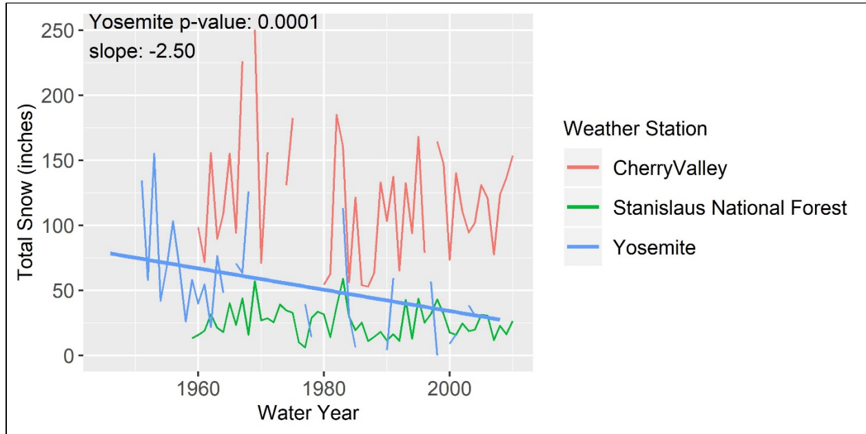
Figure 3. Total snowfall for local Stanislaus National Forest weather stations (identified in different colors). Linear lines indicate a significant trend. For all significant trends the level of significance (p-value) and magnitude and direction of trend (slope) are presented. *Note that data for the Stanislaus National Forest (Terra Climate) are Snow Water Equivalent (in inches), while data for the individual weather stations are Total Snow (in inches).
