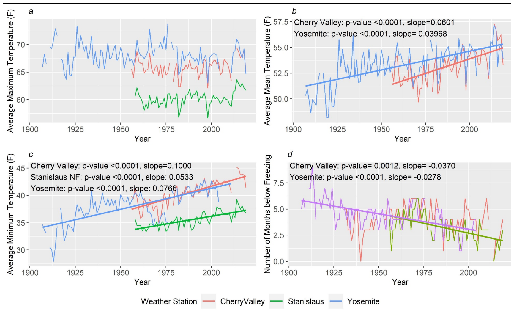
Figure 1. Historic temperature trends for Stanislaus National Forest weather stations (identified in different colors): a) Average Maximum Temperature, b) Average Mean Temperature, c) Average Minimum Temperature, and D) Number of Months below Freezing (months where the average minimum temperature was <32°F). Linear lines indicate a significant trend. For all significant trends the level of significance (p-value) and magnitude and direction of trend (slope) are presented.
