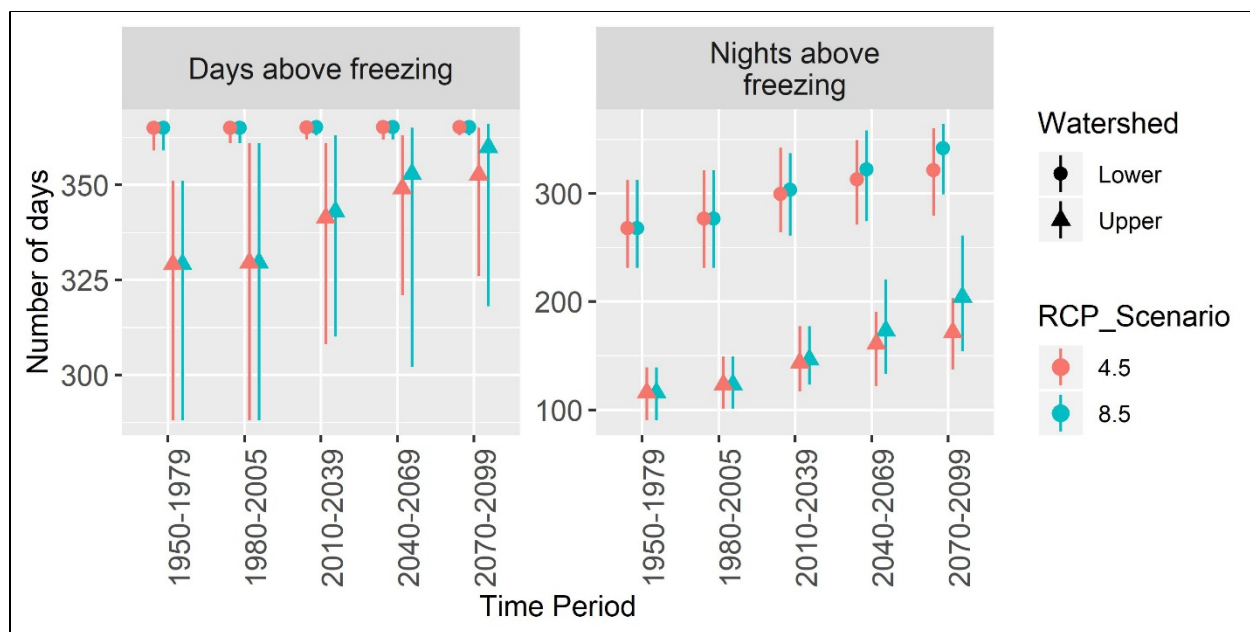
Figure 12. Modeled number of days above freezing (32°F) for the Clark Fork Watershed and Big Creek-Tuolumne River Watershed on the Stanislaus National Forest summarized for 30-year periods. Points represent the average while lines indicate range of data. Data source CalAdapt: See Table 4 footnote. Days above freezing and nights above freezing are based on when the daily maximum/minimum exceeds 32°F.
