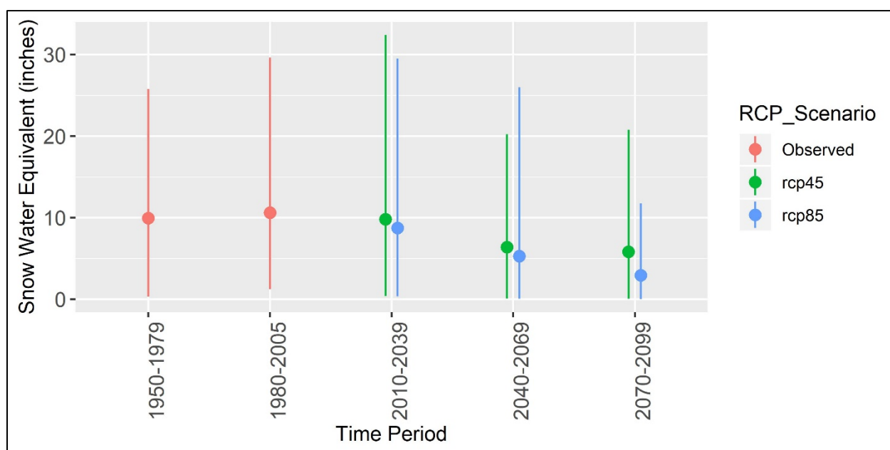
Figure 17: Historic observed and future predicted April 1 st Snow Water Equivalent (SWE) on the Stanislaus National Forest summarized for 30-year periods under two emission scenarios (RCP 4.5 and RCP 8.5). Points represent average while lines indicate range of data (minimum and maximum). Data source CalAdapt: See Table 4 footnote.
