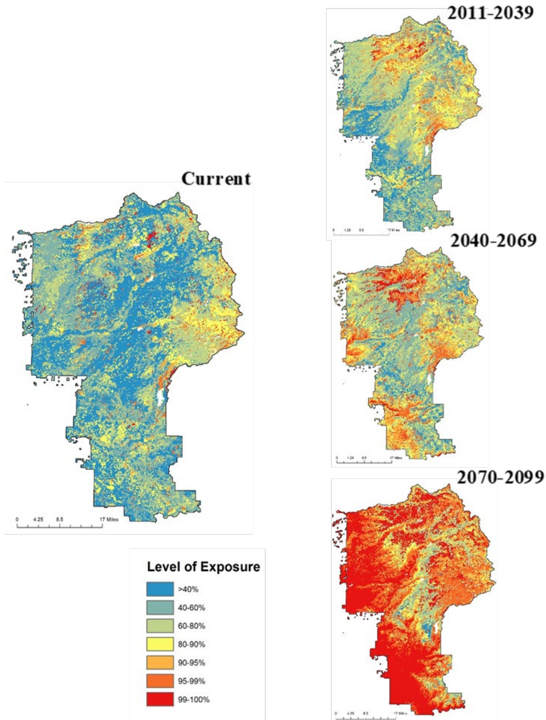
Figure 22. Mapped climate exposure under the “Warm and Wet” CNRM CM5 climate projection under Higher Emissions RCP8.5. This image shows the climate exposure of Stanislaus National Forest vegetation types at current time and three future periods: 2011–2039, 2040–2069, and 2070–2099. Areas considered to be highly climatically exposed are in the 95–99% and 99–100%. Areas with values <80% are considered to be in climatically suitable conditions for the vegetation that it currently occupies.
